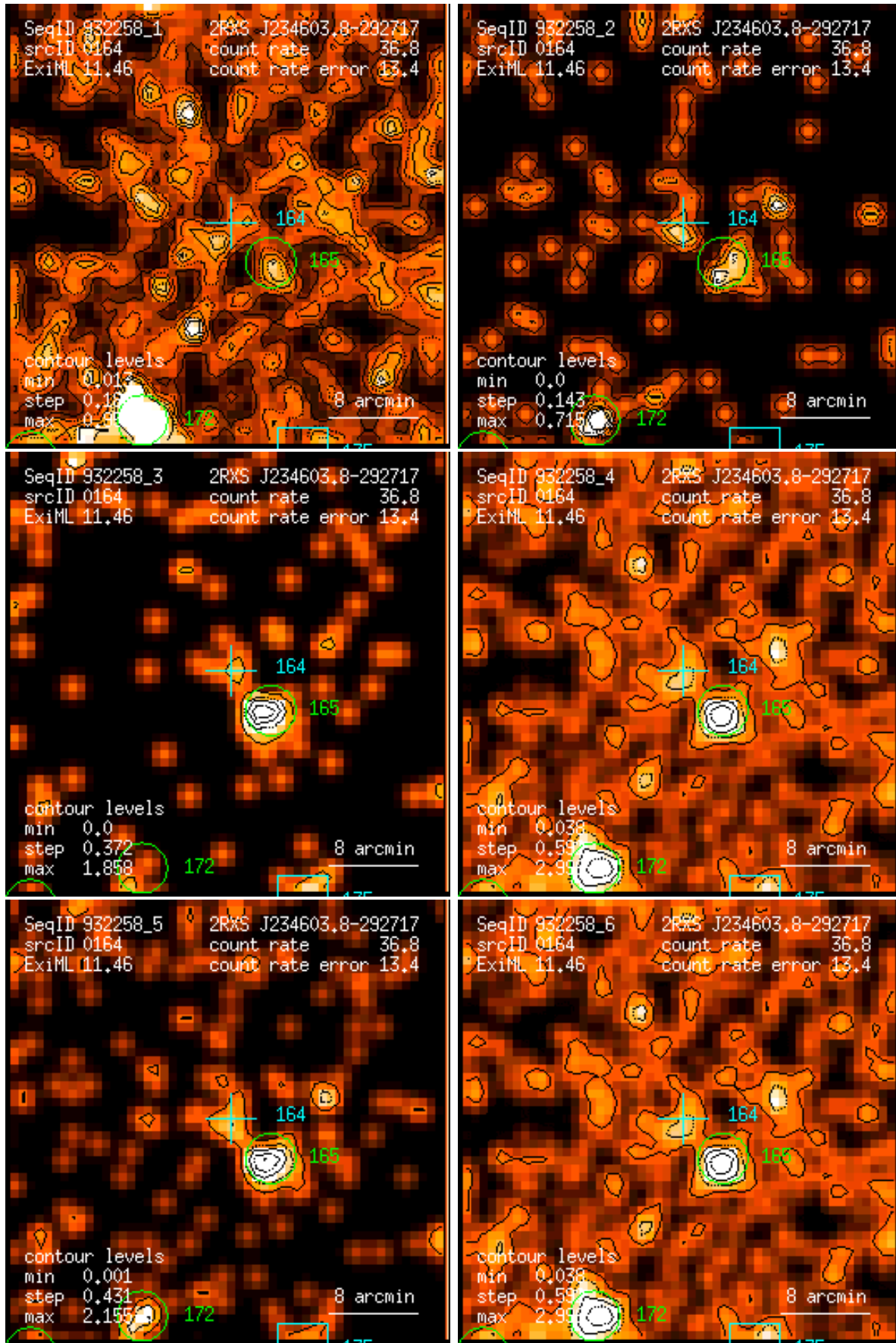
Figure 164: RASS 932258: detection 0164: band rate images, Gaussian filter: (1) PSPC channels 11 – 41, (2) 52 – 90, (3) 91 – 201, (4) 11 – 235, (5) 52 – 201, (6) 11 – 201. Broad band rates in counts/ks. Band rate contour levels in counts/ks/arcmin 2 .
