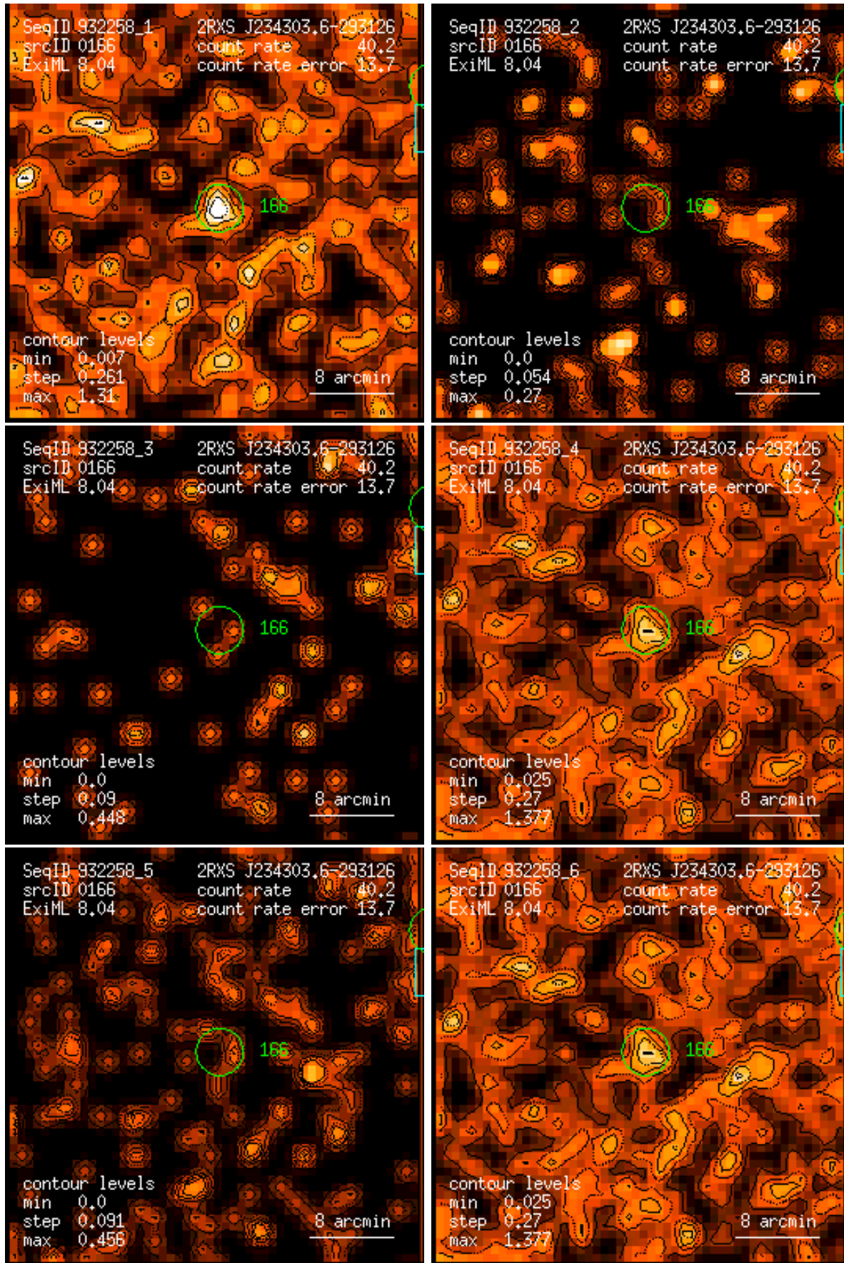
Figure 166: RASS 932258: detection 0166: band rate images, Gaussian filter: (1) PSPC channels 11 – 41, (2) 52 – 90, (3) 91 – 201, (4) 11 – 235, (5) 52 – 201, (6) 11 – 201. Broad band rates in counts/ks. Band rate contour levels in counts/ks/arcmin 2 .
