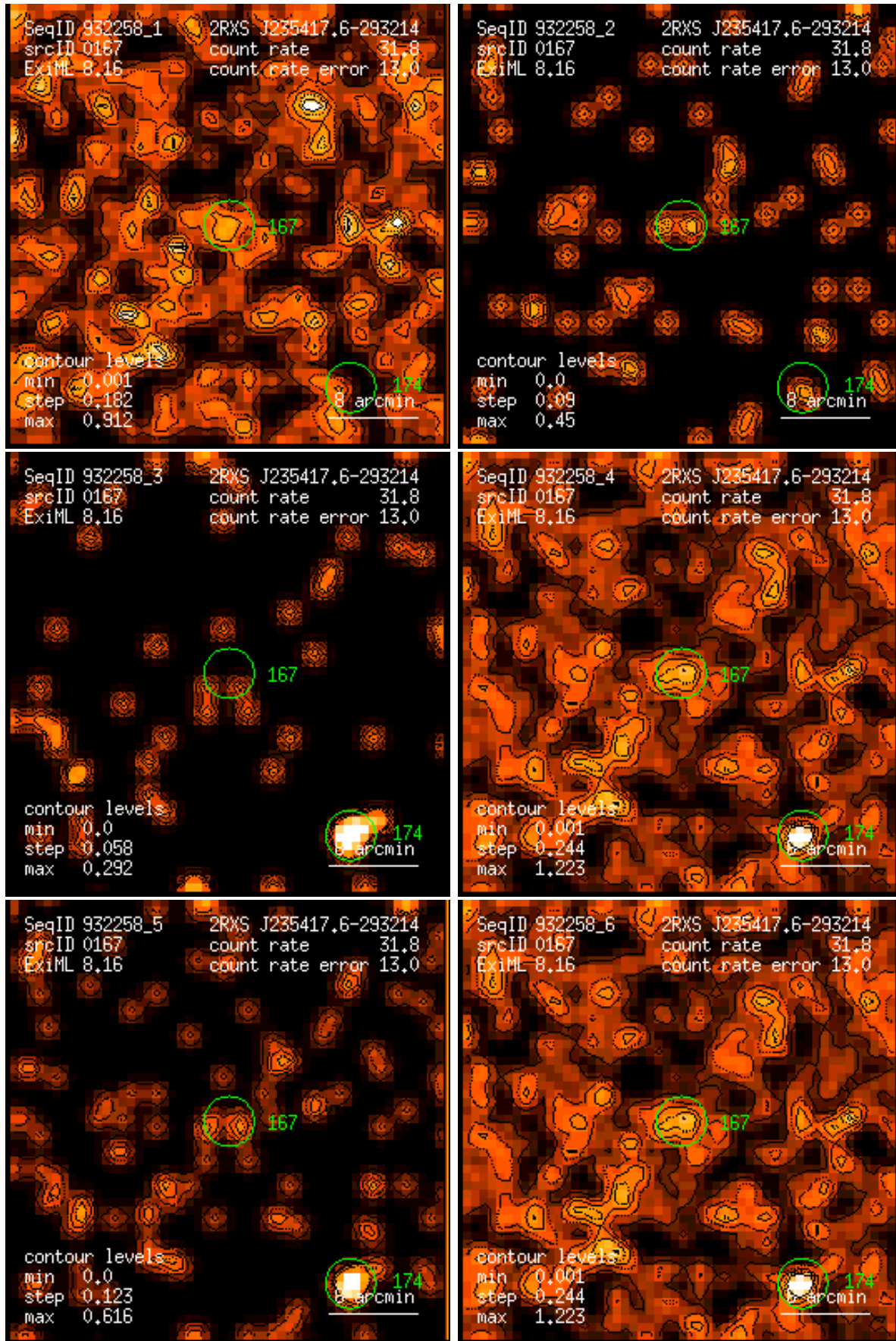
Figure 167: RASS 932258: detection 0167: band rate images, Gaussian filter: (1) PSPC channels 11 – 41, (2) 52 – 90, (3) 91 – 201, (4) 11 – 235, (5) 52 – 201, (6) 11 – 201. Broad band rates in counts/ks. Band rate contour levels in counts/ks/arcmin 2 .
