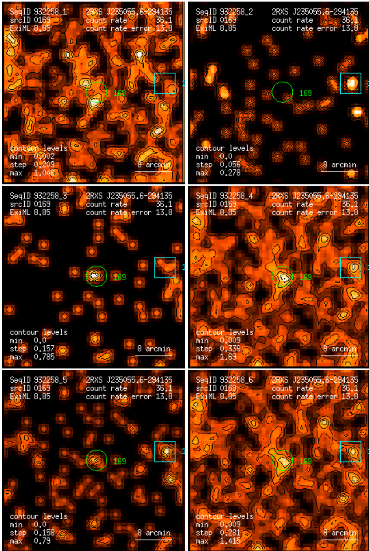
Figure 169: RASS 932258: detection 0169: band rate images, Gaussian filter: (1) PSPC channels 11 – 41, (2) 52 – 90, (3) 91 – 201, (4) 11 – 235, (5) 52 – 201, (6) 11 – 201. Broad band rates in counts/ks. Band rate contour levels in counts/ks/arcmin 2 .
