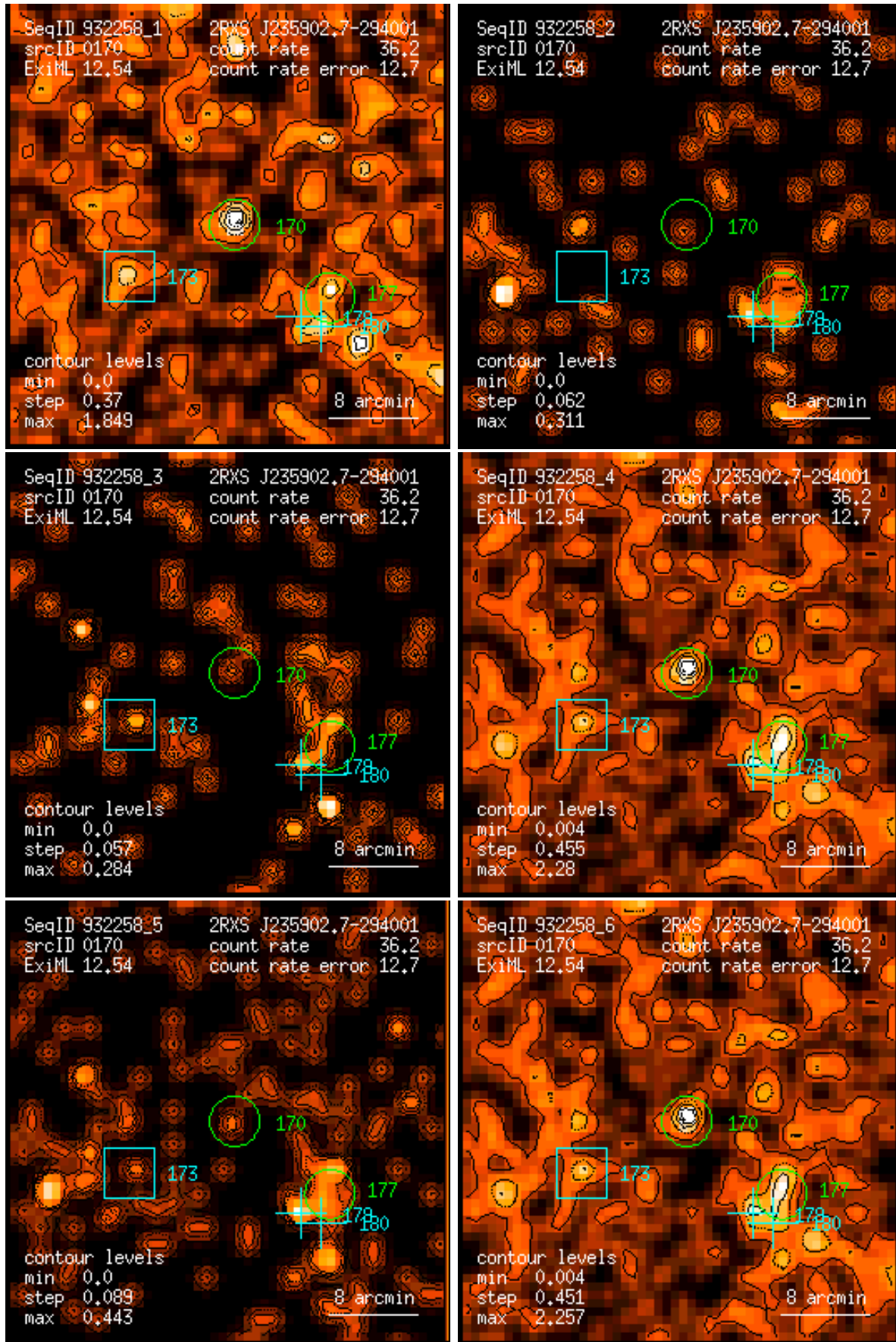
Figure 170: RASS 932258: detection 0170: band rate images, Gaussian filter: (1) PSPC channels 11 – 41, (2) 52 – 90, (3) 91 – 201, (4) 11 – 235, (5) 52 – 201, (6) 11 – 201. Broad band rates in counts/ks. Band rate contour levels in counts/ks/arcmin 2 .
