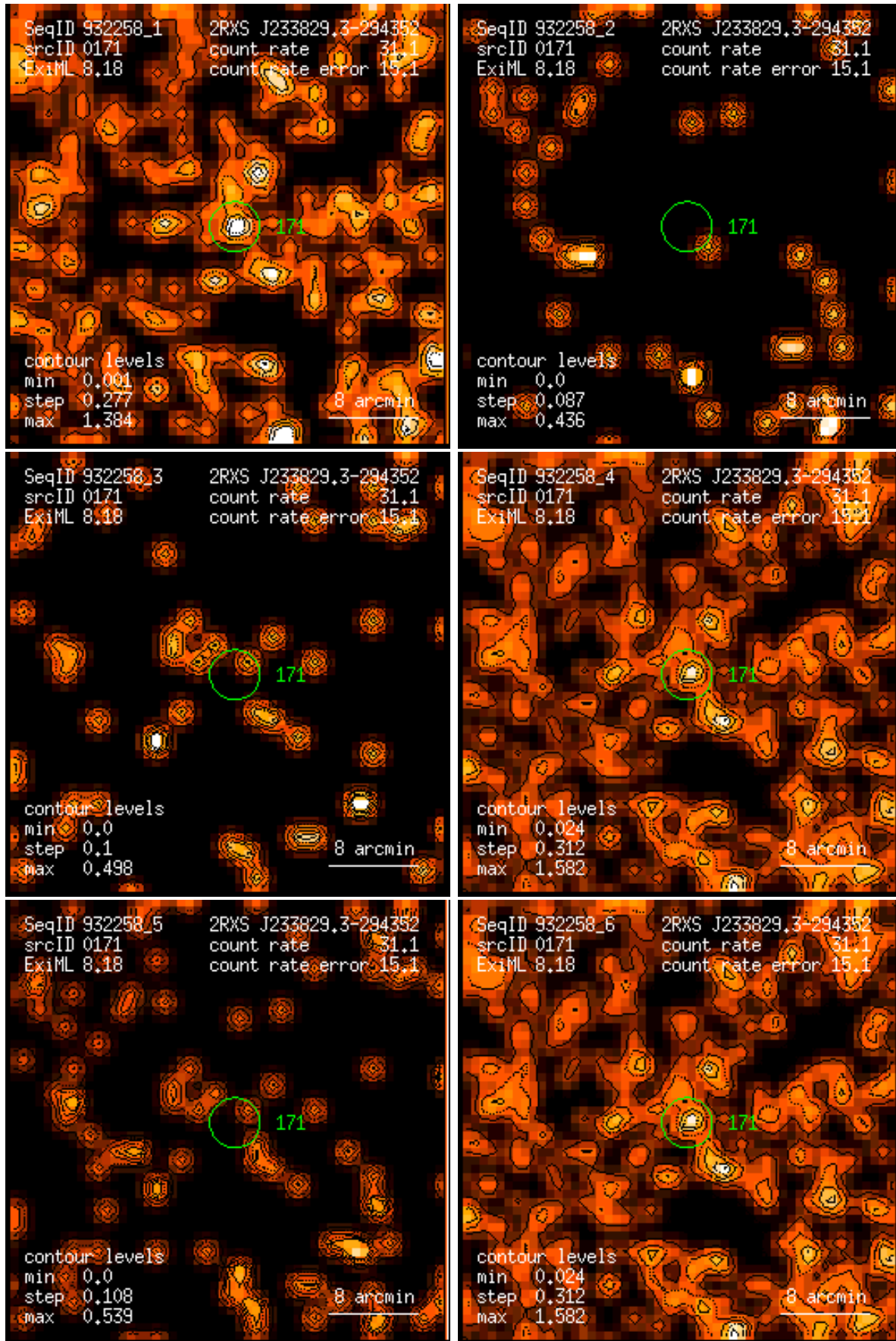
Figure 171: RASS 932258: detection 0171: band rate images, Gaussian filter: (1) PSPC channels 11 – 41, (2) 52 – 90, (3) 91 – 201, (4) 11 – 235, (5) 52 – 201, (6) 11 – 201. Broad band rates in counts/ks. Band rate contour levels in counts/ks/arcmin 2 .
