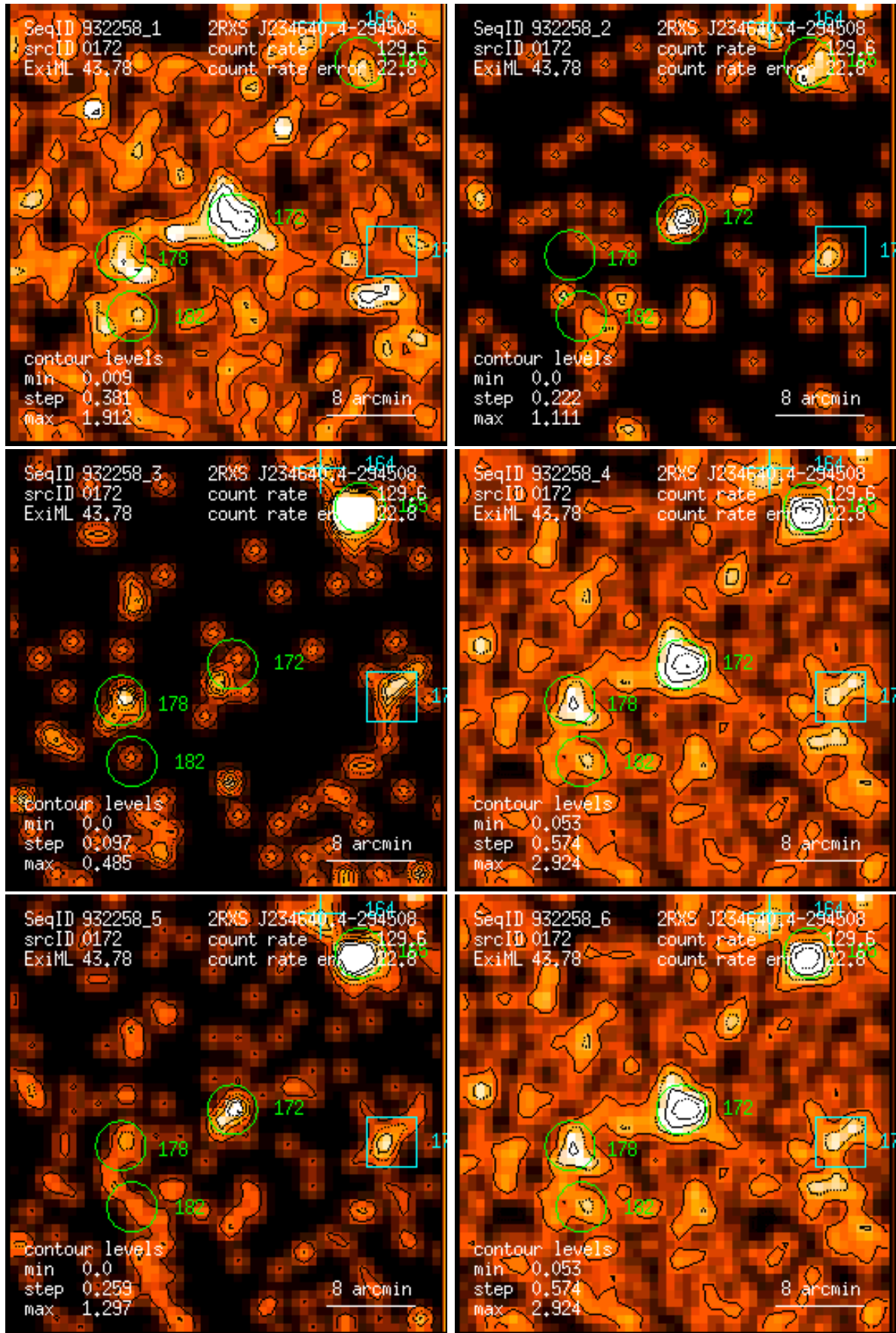
Figure 172: RASS 932258: detection 0172: band rate images, Gaussian filter: (1) PSPC channels 11 – 41, (2) 52 – 90, (3) 91 – 201, (4) 11 – 235, (5) 52 – 201, (6) 11 – 201. Broad band rates in counts/ks. Band rate contour levels in counts/ks/arcmin 2 .
