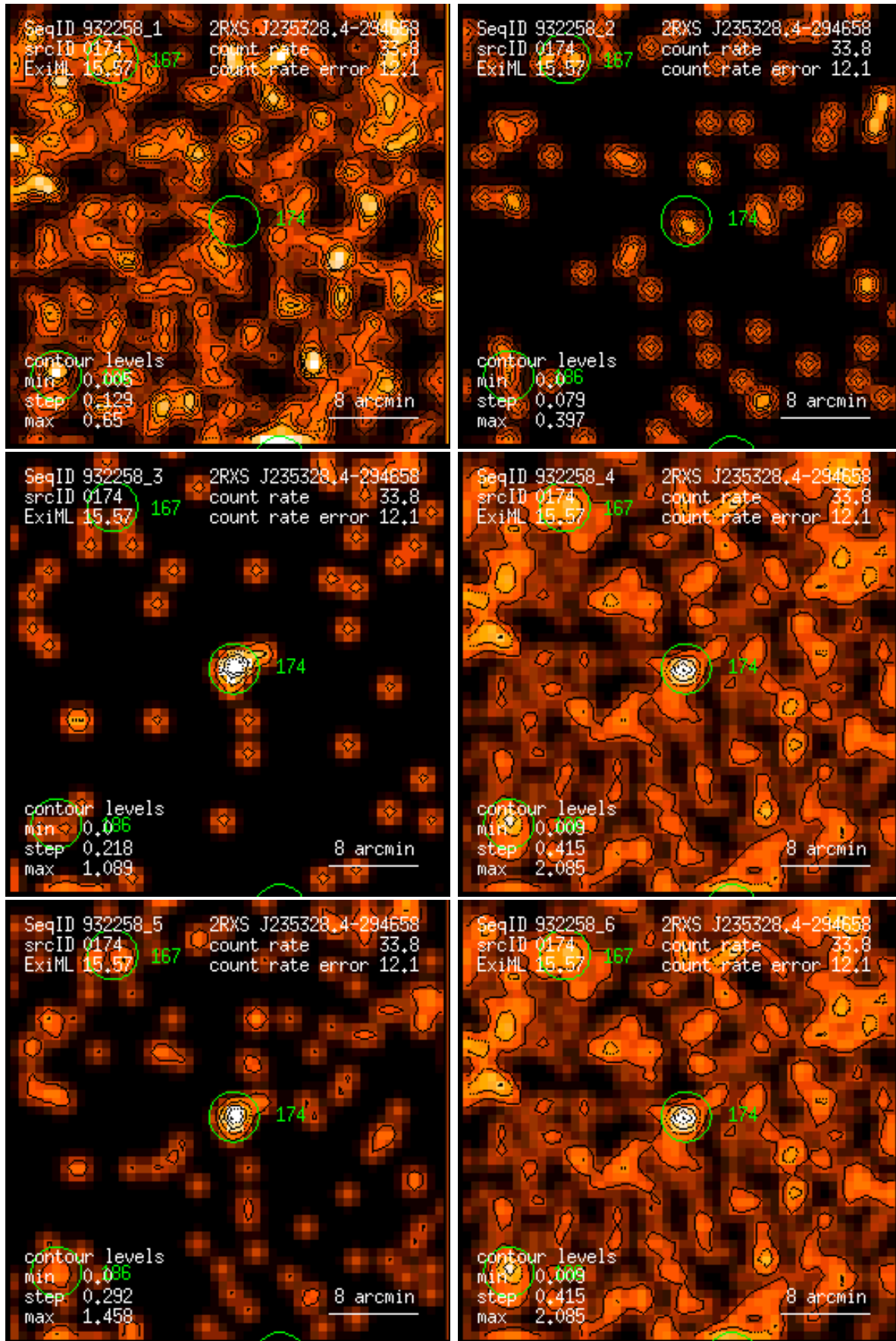
Figure 174: RASS 932258: detection 0174: band rate images, Gaussian filter: (1) PSPC channels 11 – 41, (2) 52 – 90, (3) 91 – 201, (4) 11 – 235, (5) 52 – 201, (6) 11 – 201. Broad band rates in counts/ks. Band rate contour levels in counts/ks/arcmin 2 .
