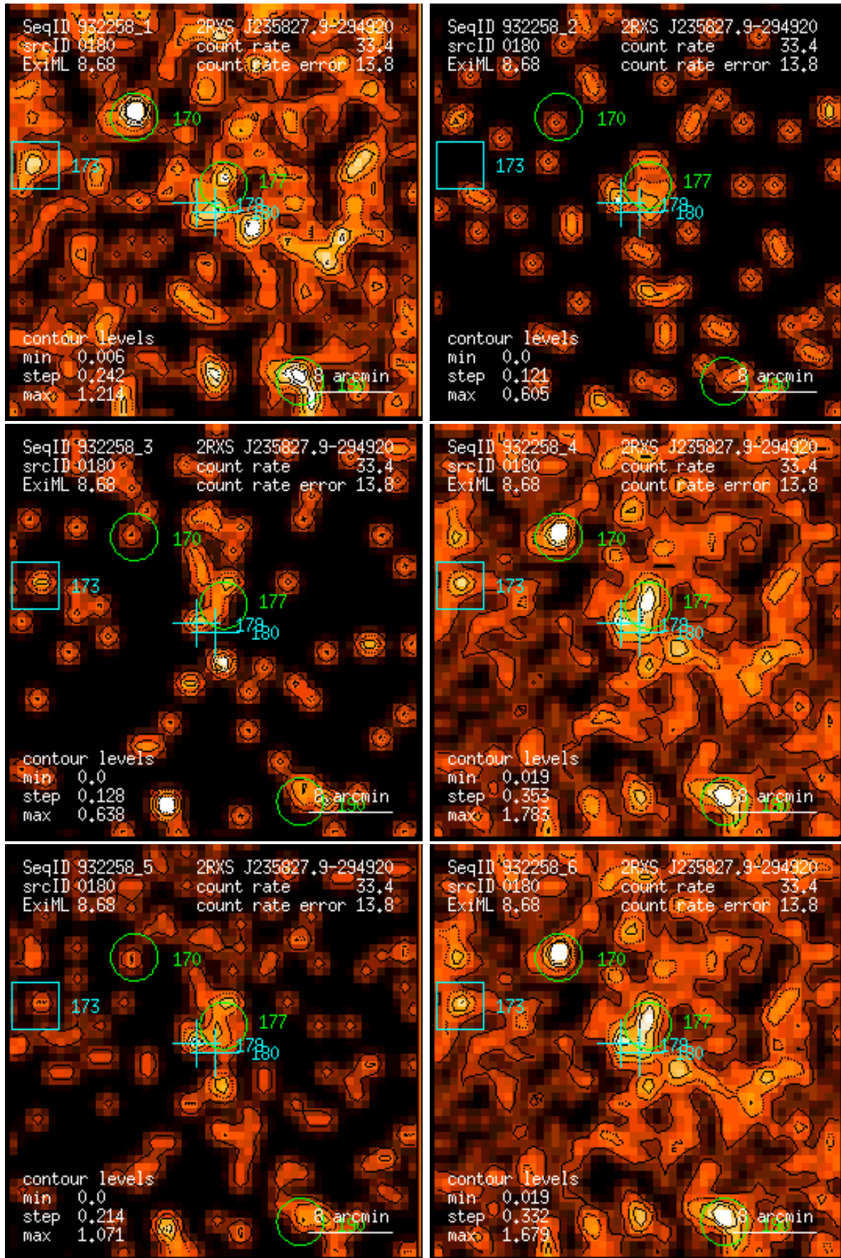
Figure 180: RASS 932258: detection 0180: band rate images, Gaussian filter: (1) PSPC channels 11 – 41, (2) 52 – 90, (3) 91 – 201, (4) 11 – 235, (5) 52 – 201, (6) 11 – 201. Broad band rates in counts/ks. Band rate contour levels in counts/ks/arcmin 2 .
