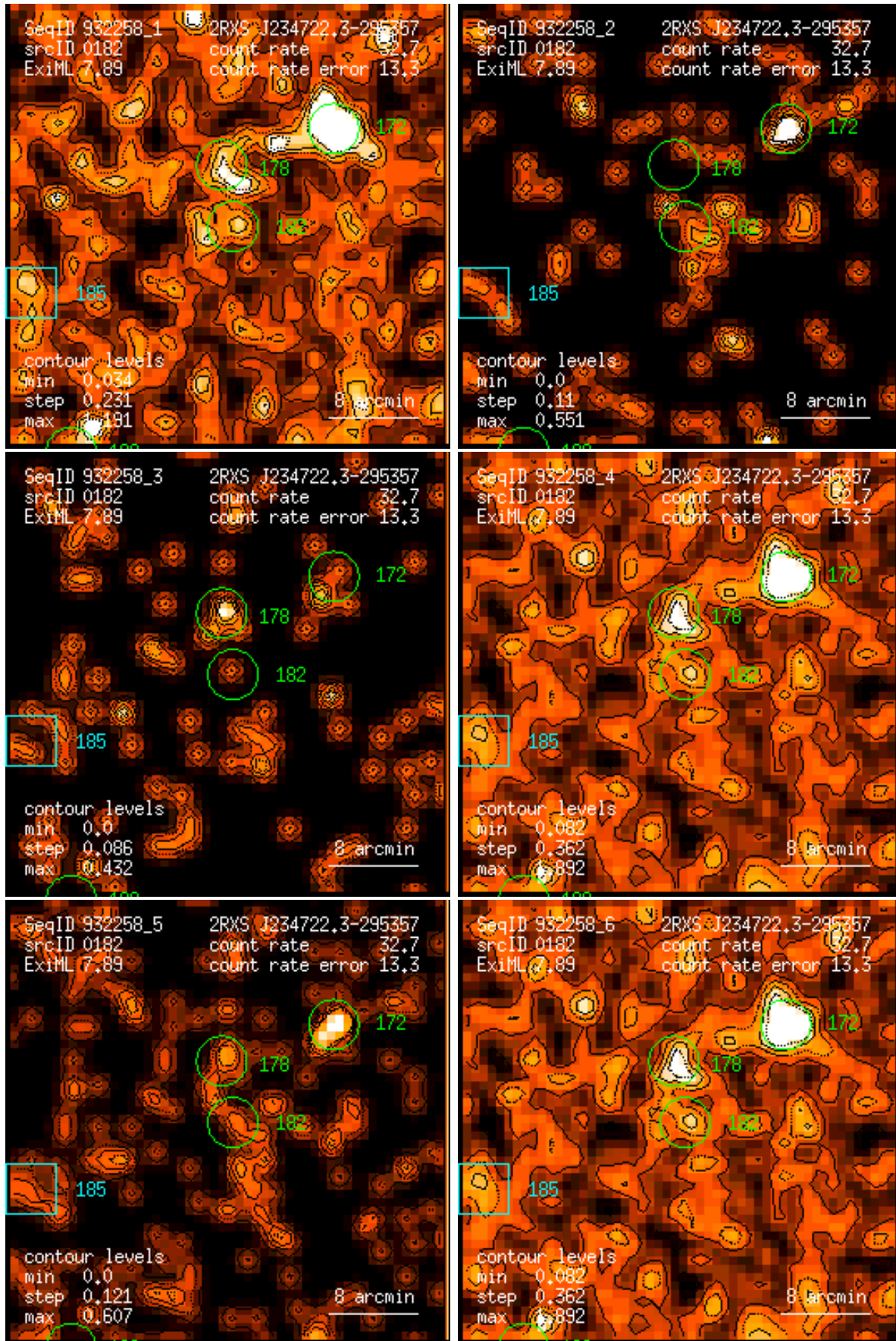
Figure 182: RASS 932258: detection 0182: band rate images, Gaussian filter: (1) PSPC channels 11 – 41, (2) 52 – 90, (3) 91 – 201, (4) 11 – 235, (5) 52 – 201, (6) 11 – 201. Broad band rates in counts/ks. Band rate contour levels in counts/ks/arcmin 2 .
