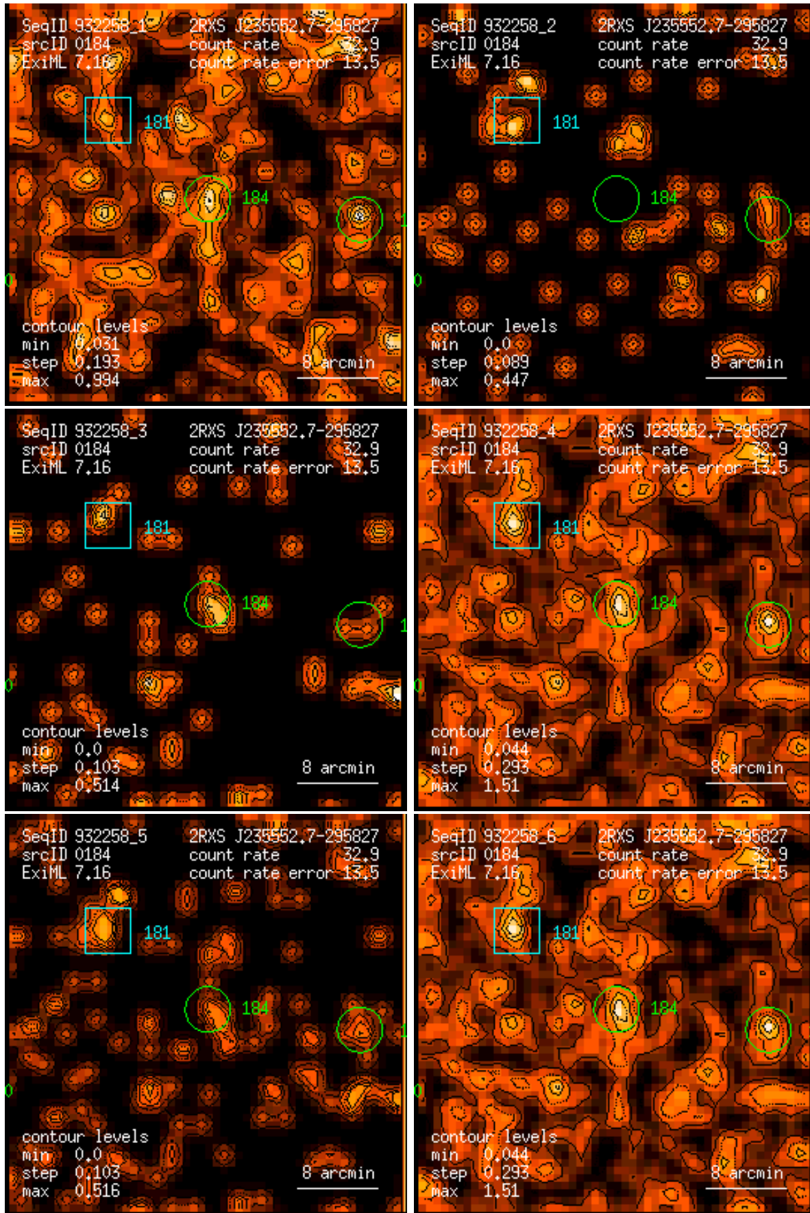
Figure 184: RASS 932258: detection 0184: band rate images, Gaussian filter: (1) PSPC channels 11 – 41, (2) 52 – 90, (3) 91 – 201, (4) 11 – 235, (5) 52 – 201, (6) 11 – 201. Broad band rates in counts/ks. Band rate contour levels in counts/ks/arcmin 2 .
