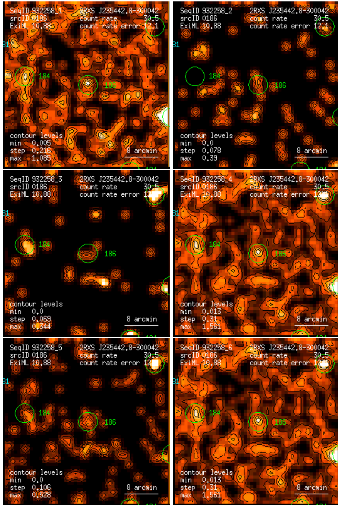
Figure 186: RASS 932258: detection 0186: band rate images, Gaussian filter: (1) PSPC channels 11 – 41, (2) 52 – 90, (3) 91 – 201, (4) 11 – 235, (5) 52 – 201, (6) 11 – 201. Broad band rates in counts/ks. Band rate contour levels in counts/ks/arcmin 2 .
