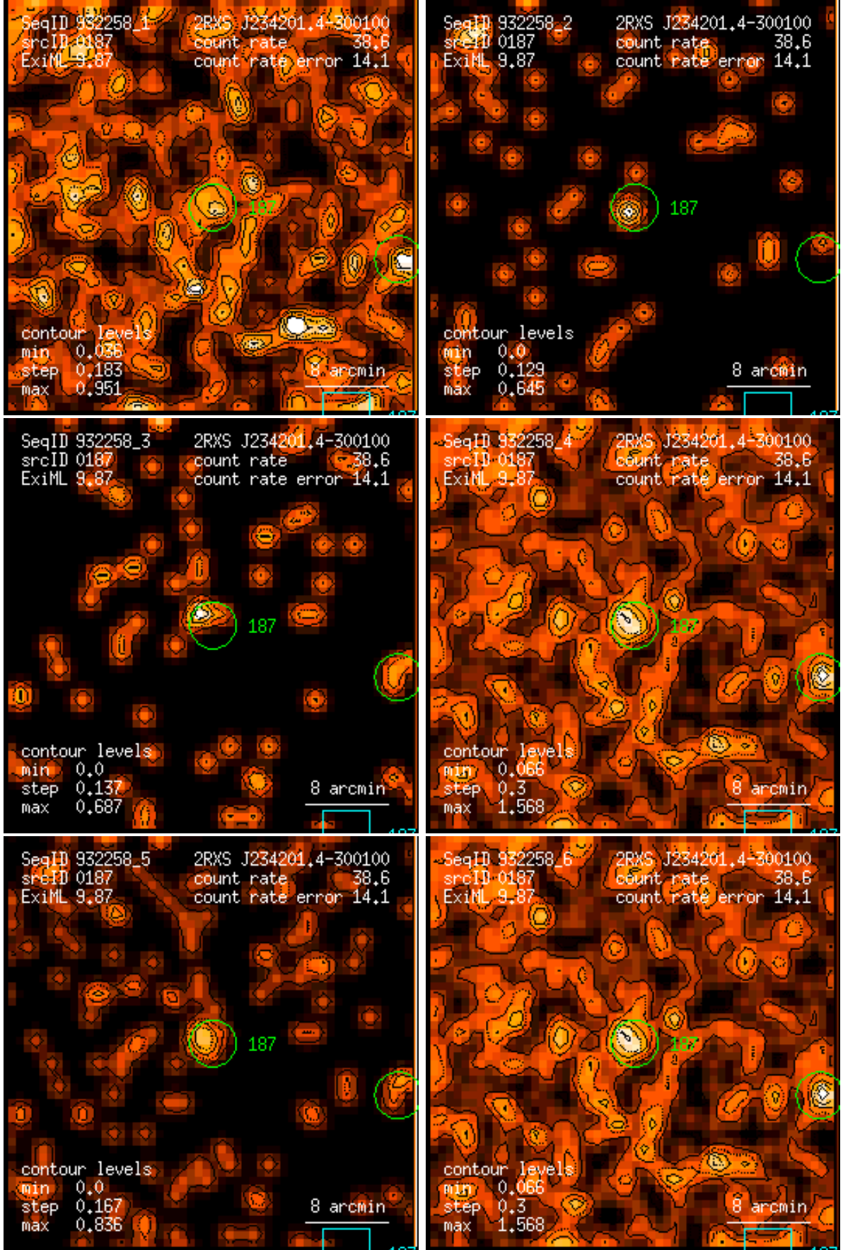
Figure 187: RASS 932258: detection 0187: band rate images, Gaussian filter: (1) PSPC channels 11 – 41, (2) 52 – 90, (3) 91 – 201, (4) 11 – 235, (5) 52 – 201, (6) 11 – 201. Broad band rates in counts/ks. Band rate contour levels in counts/ks/arcmin 2 .
