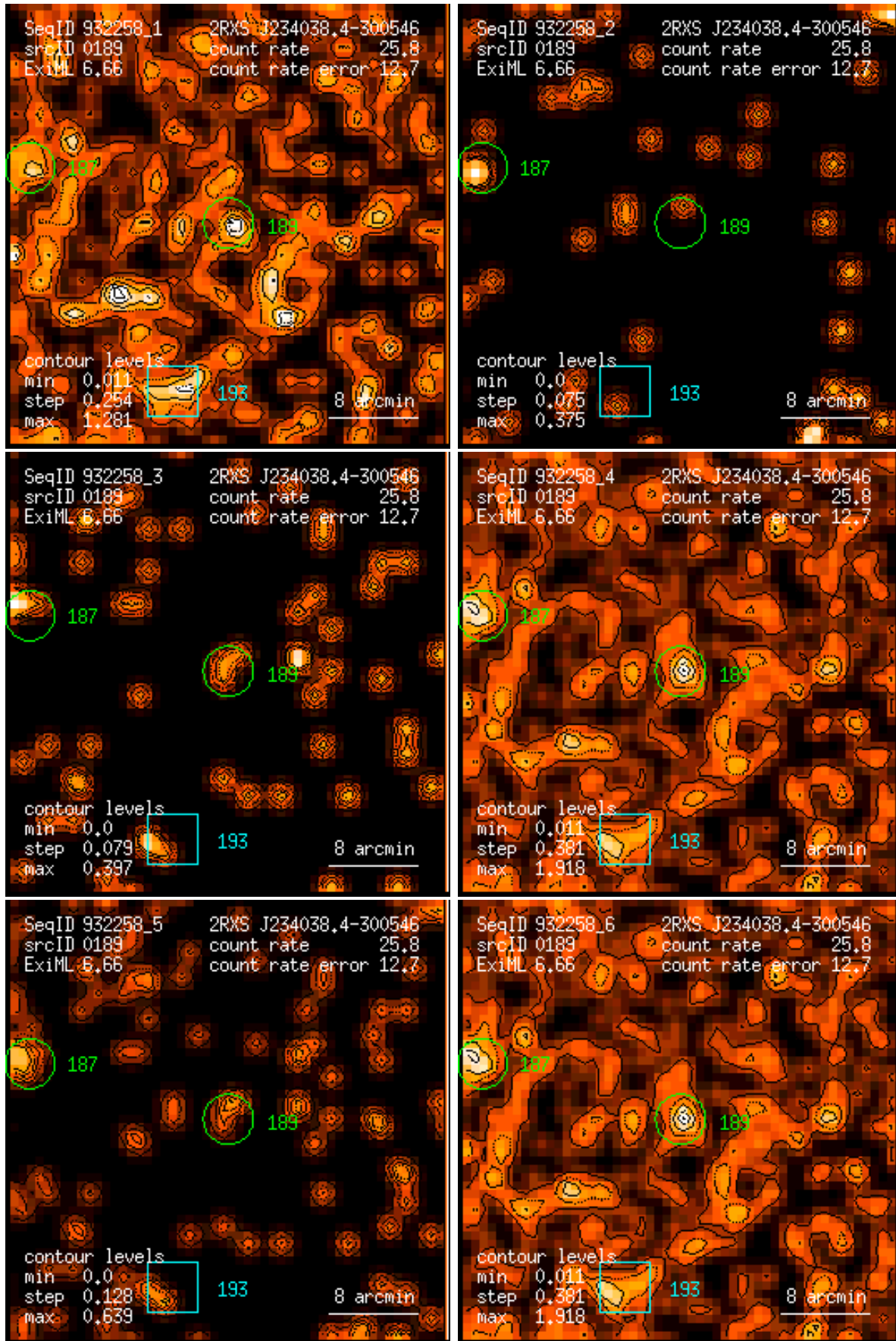
Figure 189: RASS 932258: detection 0189: band rate images, Gaussian filter: (1) PSPC channels 11 – 41, (2) 52 – 90, (3) 91 – 201, (4) 11 – 235, (5) 52 – 201, (6) 11 – 201. Broad band rates in counts/ks. Band rate contour levels in counts/ks/arcmin 2 .
