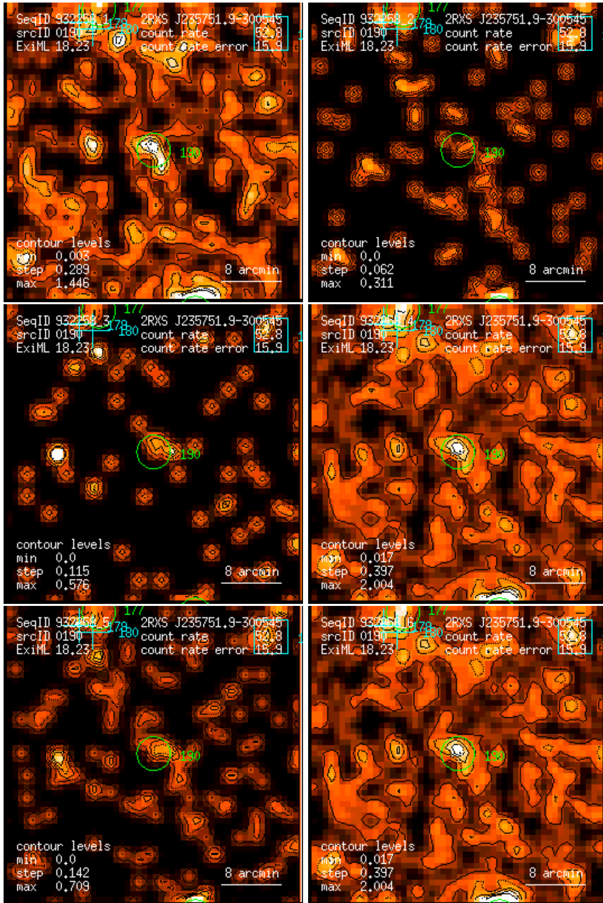
Figure 190: RASS 932258: detection 0190: band rate images, Gaussian filter: (1) PSPC channels 11 – 41, (2) 52 – 90, (3) 91 – 201, (4) 11 – 235, (5) 52 – 201, (6) 11 – 201. Broad band rates in counts/ks. Band rate contour levels in counts/ks/arcmin 2 .
