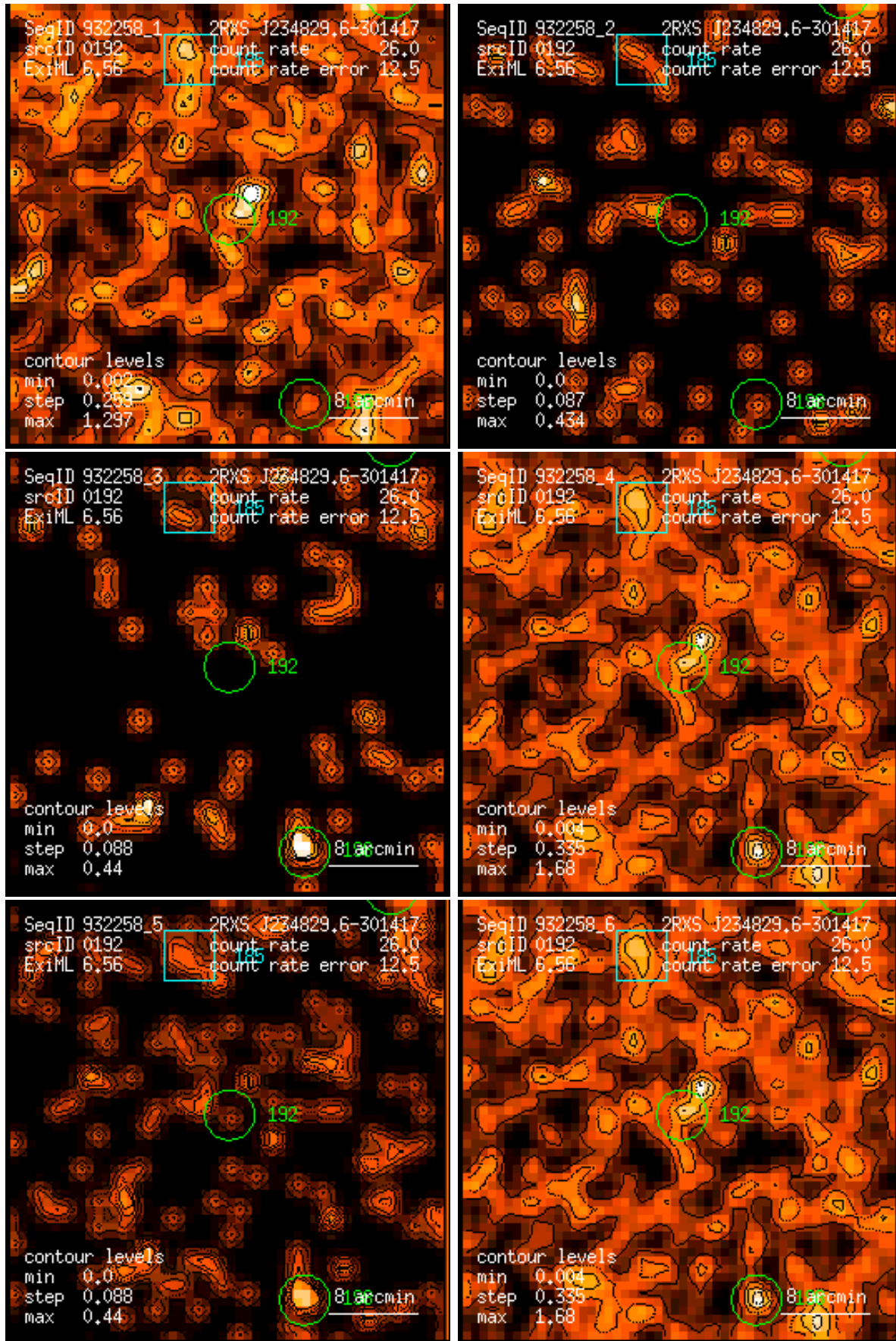
Figure 192: RASS 932258: detection 0192: band rate images, Gaussian filter: (1) PSPC channels 11 – 41, (2) 52 – 90, (3) 91 – 201, (4) 11 – 235, (5) 52 – 201, (6) 11 – 201. Broad band rates in counts/ks. Band rate contour levels in counts/ks/arcmin 2 .
