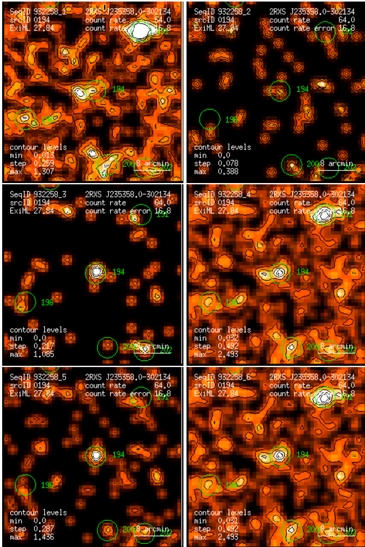
Figure 194: RASS 932258: detection 0194: band rate images, Gaussian filter: (1) PSPC channels 11 – 41, (2) 52 – 90, (3) 91 – 201, (4) 11 – 235, (5) 52 – 201, (6) 11 – 201. Broad band rates in counts/ks. Band rate contour levels in counts/ks/arcmin 2 .
