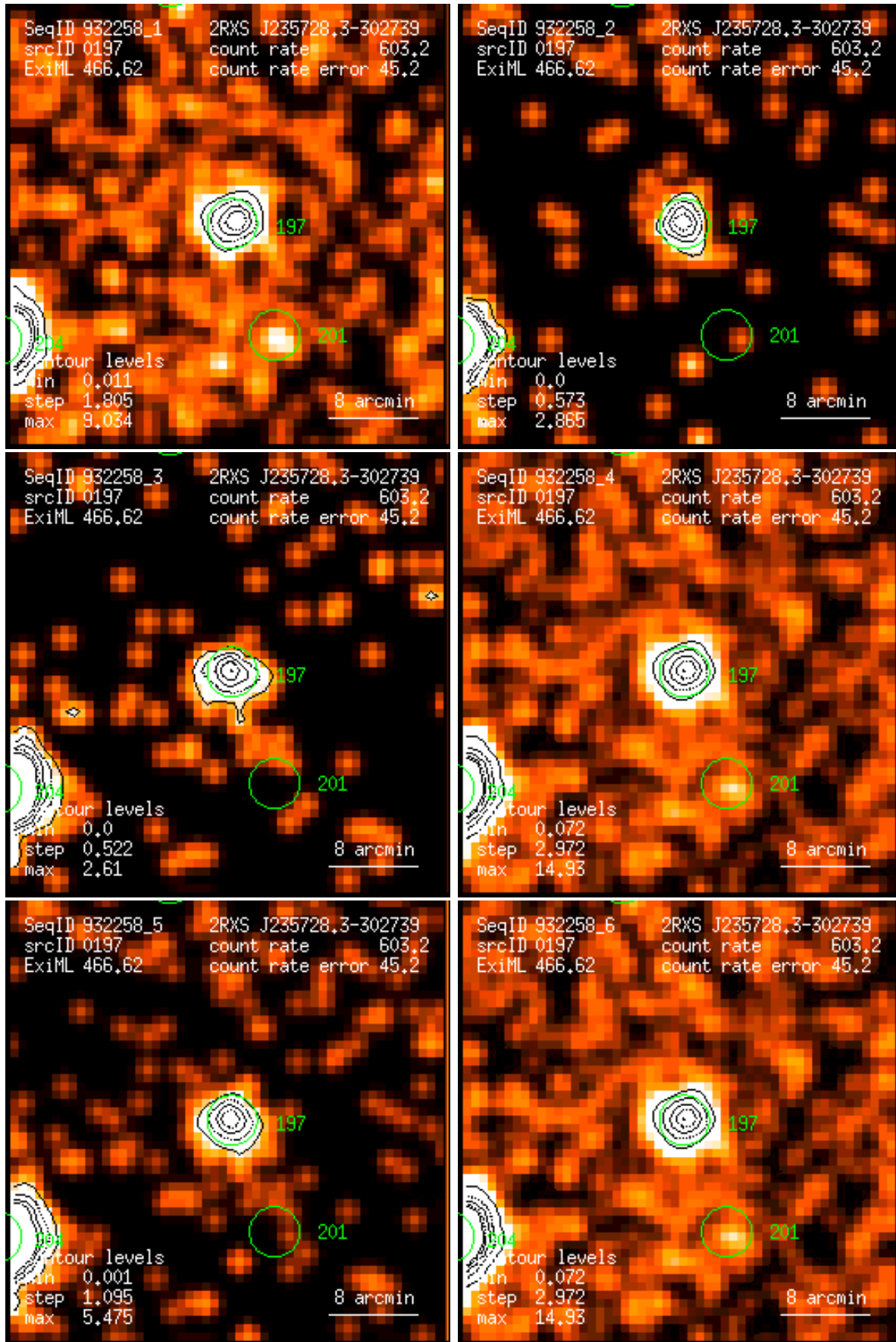
Figure 197: RASS 932258: detection 0197: band rate images, Gaussian filter: (1) PSPC channels 11 – 41, (2) 52 – 90, (3) 91 – 201, (4) 11 – 235, (5) 52 – 201, (6) 11 – 201. Broad band rates in counts/ks. Band rate contour levels in counts/ks/arcmin 2 .
