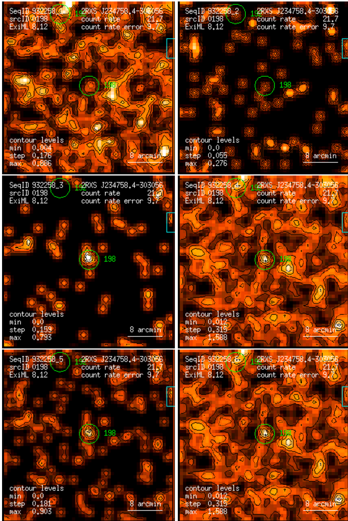
Figure 198: RASS 932258: detection 0198: band rate images, Gaussian filter: (1) PSPC channels 11 – 41, (2) 52 – 90, (3) 91 – 201, (4) 11 – 235, (5) 52 – 201, (6) 11 – 201. Broad band rates in counts/ks. Band rate contour levels in counts/ks/arcmin 2 .
