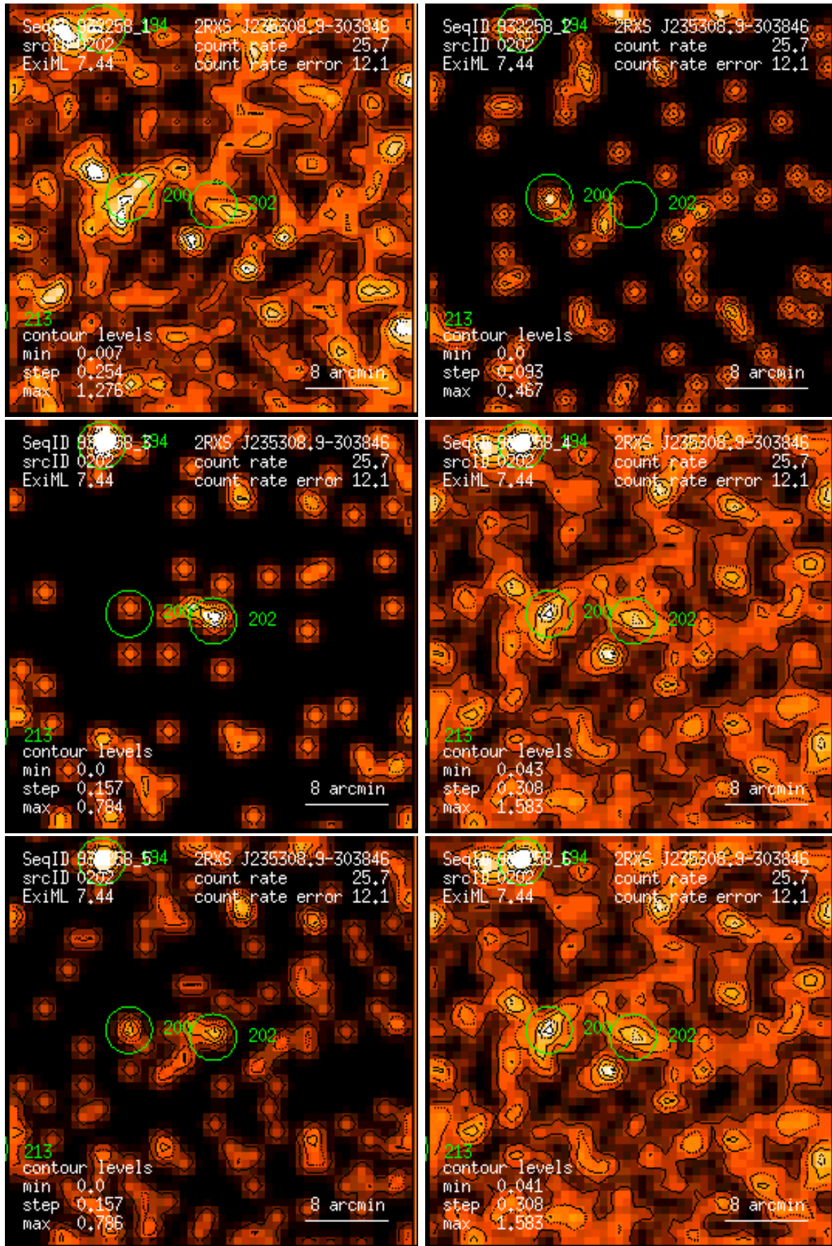
Figure 202: RASS 932258: detection 0202: band rate images, Gaussian filter: (1) PSPC channels 11 – 41, (2) 52 – 90, (3) 91 – 201, (4) 11 – 235, (5) 52 – 201, (6) 11 – 201. Broad band rates in counts/ks. Band rate contour levels in counts/ks/arcmin 2 .
