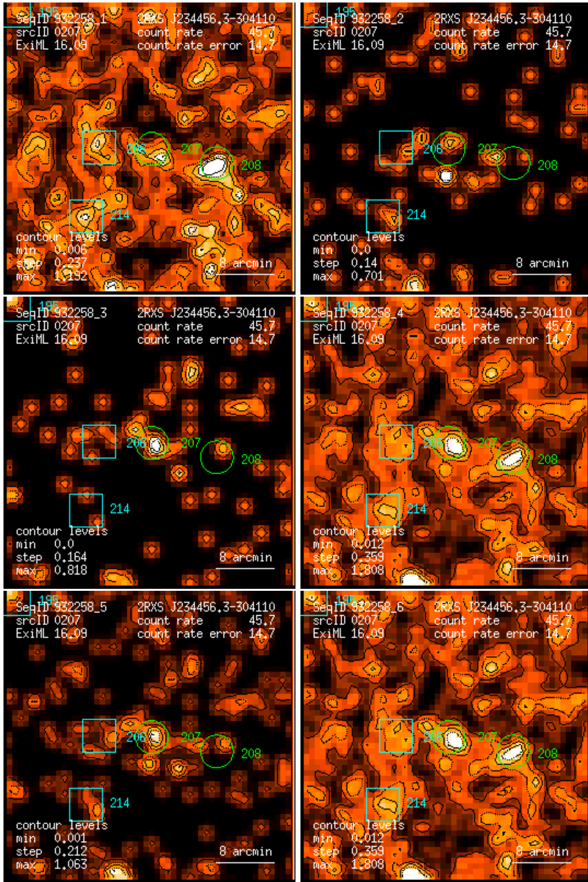
Figure 207: RASS 932258: detection 0207: band rate images, Gaussian filter: (1) PSPC channels 11 – 41, (2) 52 – 90, (3) 91 – 201, (4) 11 – 235, (5) 52 – 201, (6) 11 – 201. Broad band rates in counts/ks. Band rate contour levels in counts/ks/arcmin 2 .
