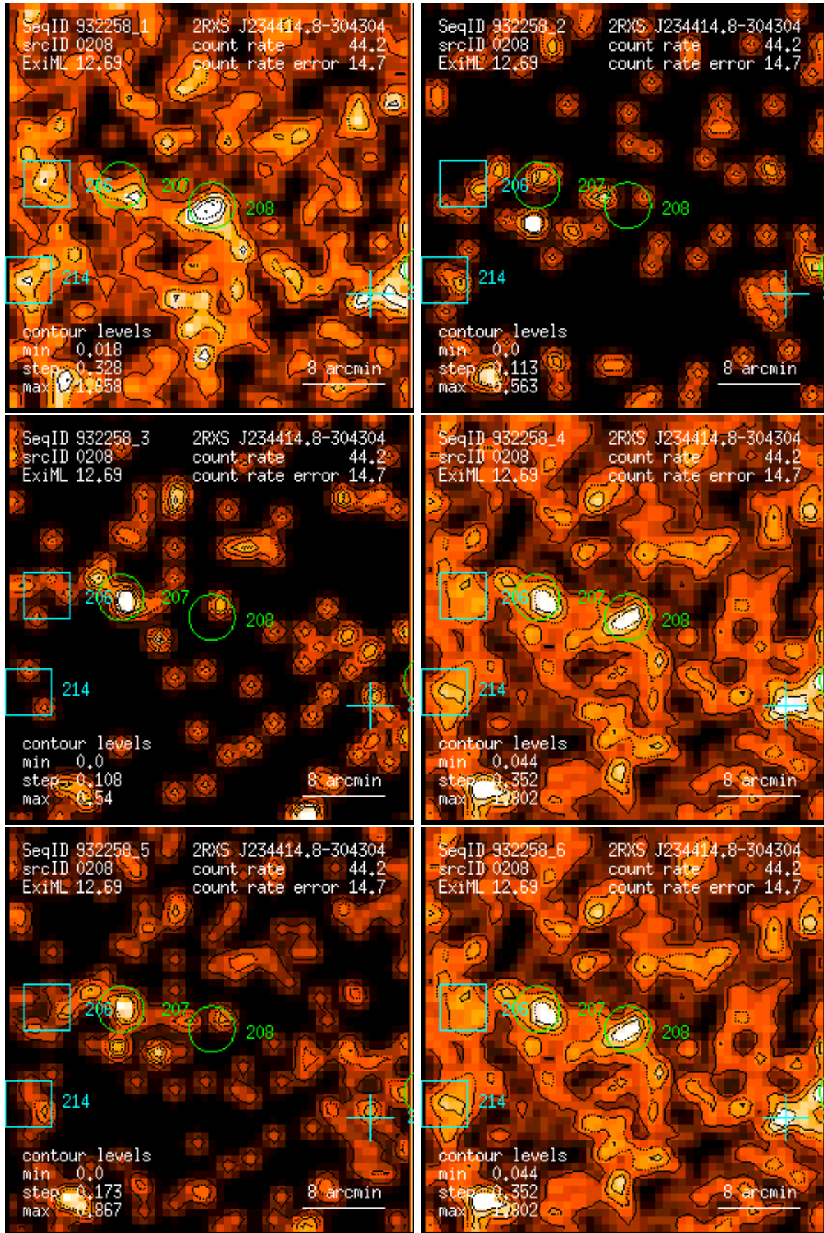
Figure 208: RASS 932258: detection 0208: band rate images, Gaussian filter: (1) PSPC channels 11 – 41, (2) 52 – 90, (3) 91 – 201, (4) 11 – 235, (5) 52 – 201, (6) 11 – 201. Broad band rates in counts/ks. Band rate contour levels in counts/ks/arcmin 2 .
