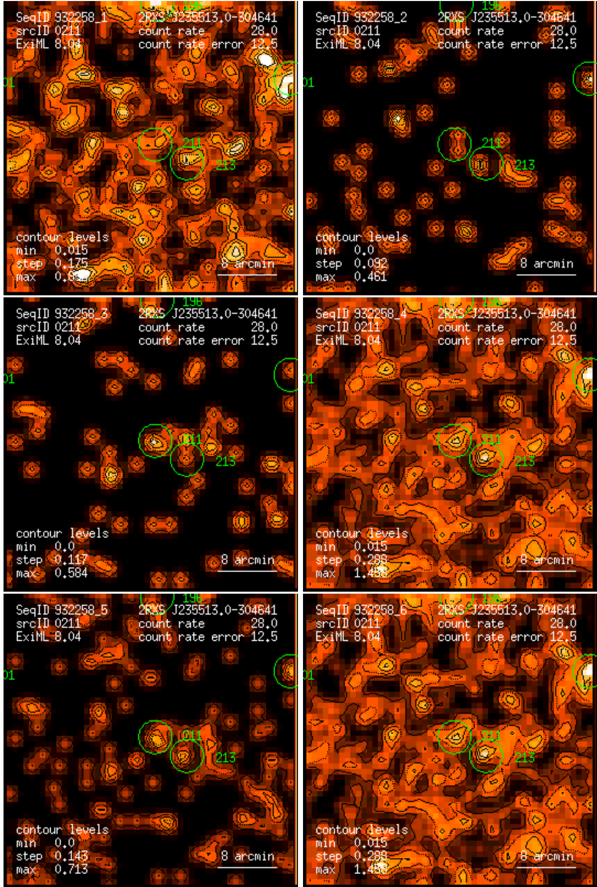
Figure 211: RASS 932258: detection 0211: band rate images, Gaussian filter: (1) PSPC channels 11 – 41, (2) 52 – 90, (3) 91 – 201, (4) 11 – 235, (5) 52 – 201, (6) 11 – 201. Broad band rates in counts/ks. Band rate contour levels in counts/ks/arcmin 2 .
