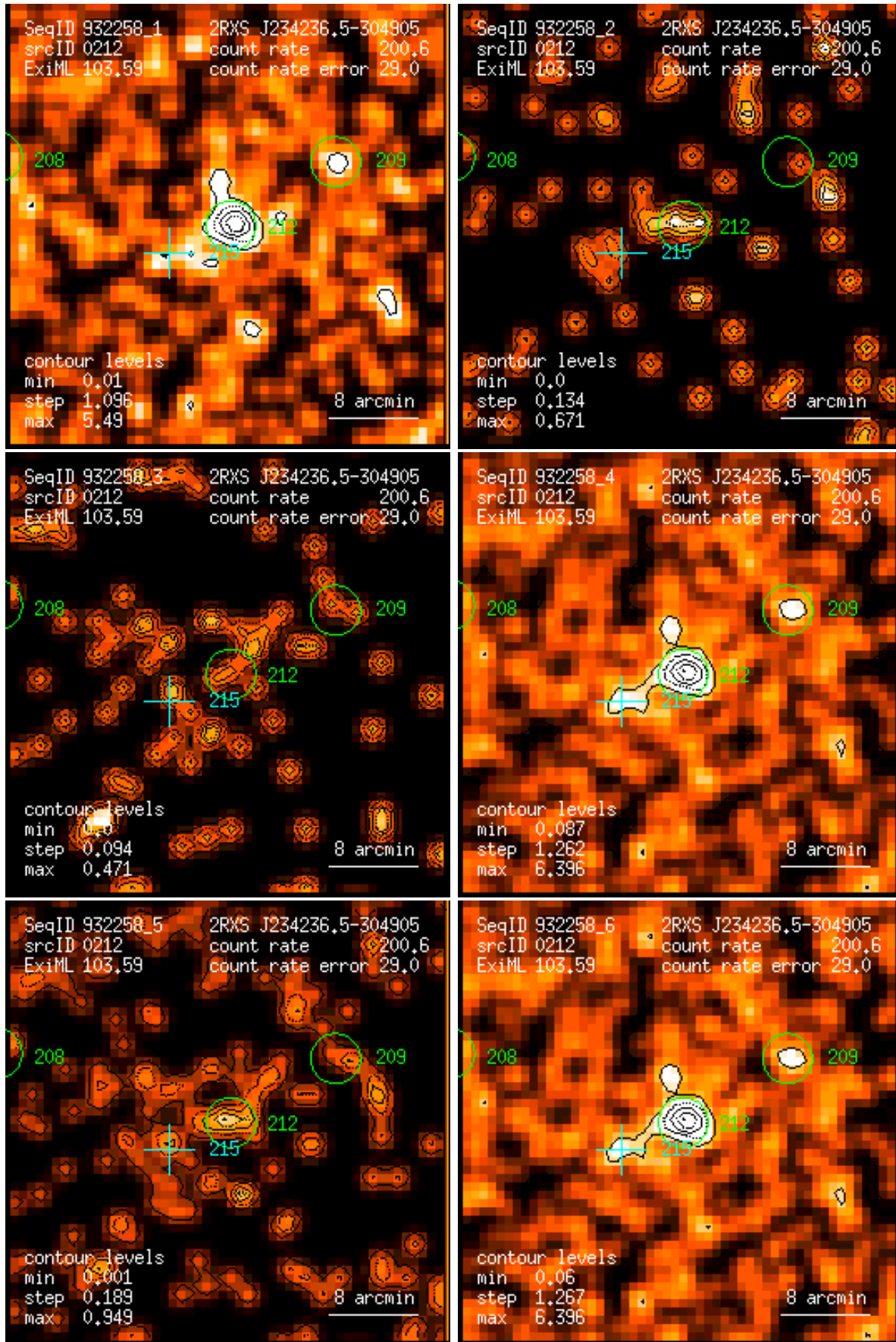
Figure 212: RASS 932258: detection 0212: band rate images, Gaussian filter: (1) PSPC channels 11 – 41, (2) 52 – 90, (3) 91 – 201, (4) 11 – 235, (5) 52 – 201, (6) 11 – 201. Broad band rates in counts/ks. Band rate contour levels in counts/ks/arcmin 2 .
