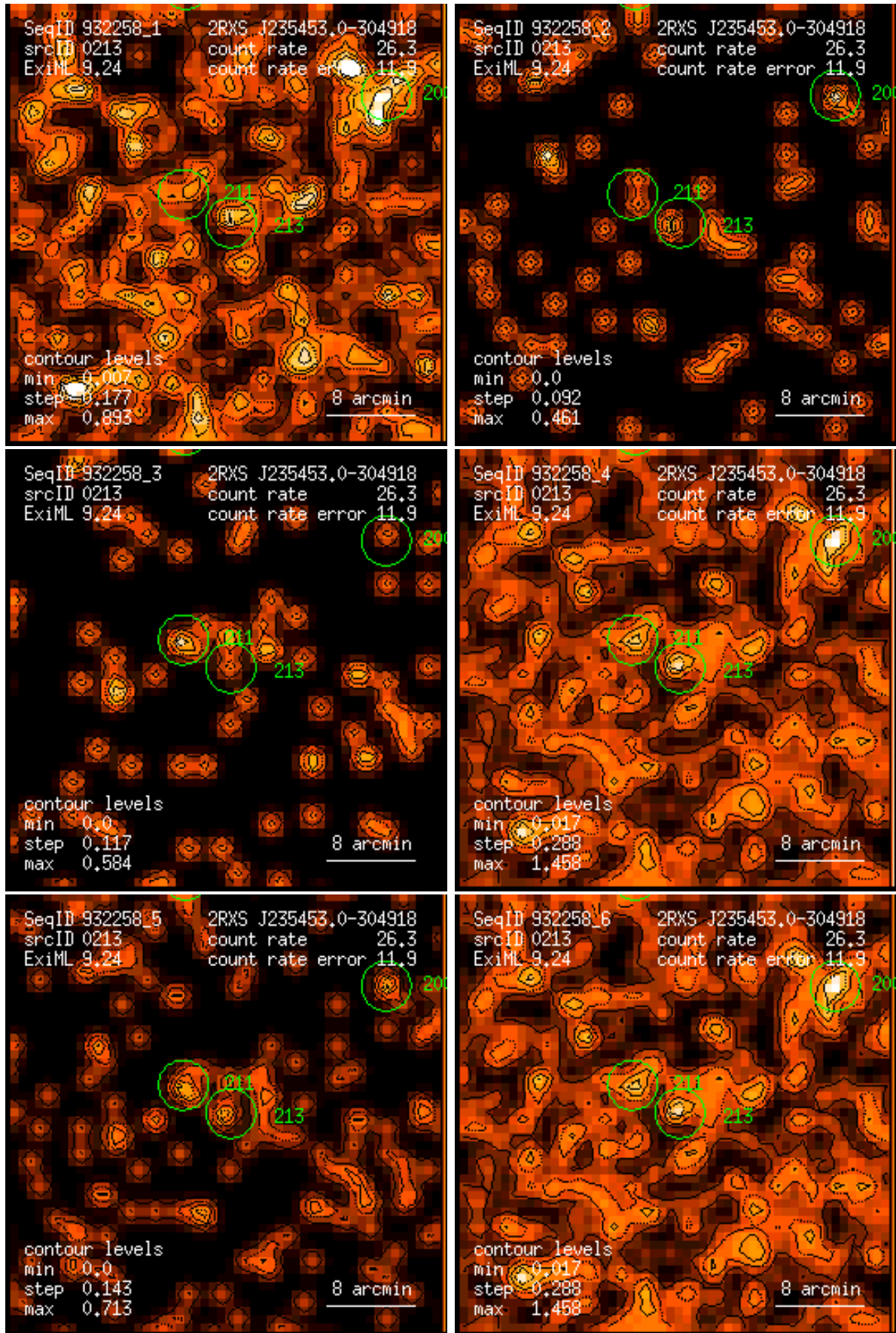
Figure 213: RASS 932258: detection 0213: band rate images, Gaussian filter: (1) PSPC channels 11 – 41, (2) 52 – 90, (3) 91 – 201, (4) 11 – 235, (5) 52 – 201, (6) 11 – 201. Broad band rates in counts/ks. Band rate contour levels in counts/ks/arcmin 2 .
