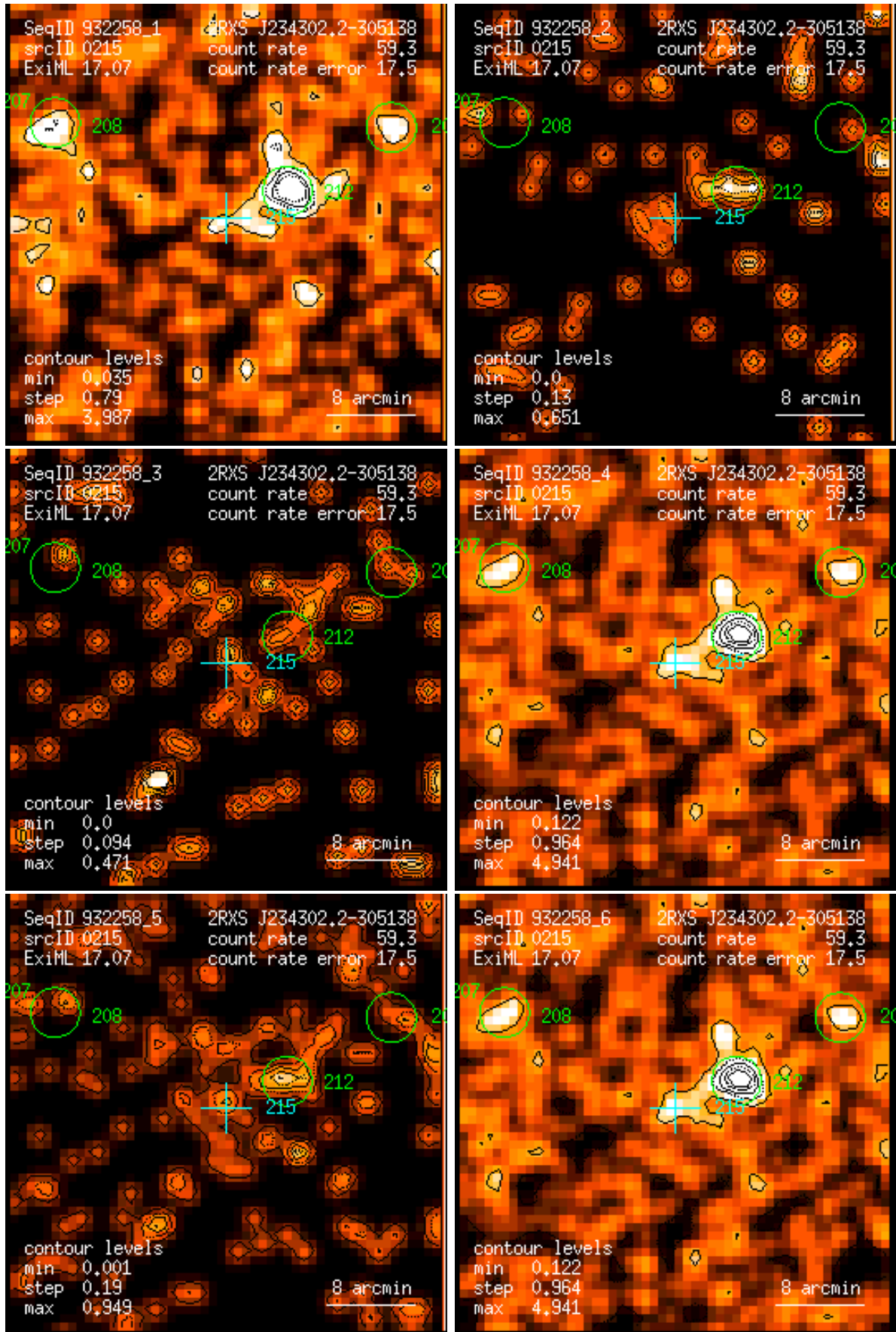
Figure 215: RASS 932258: detection 0215: band rate images, Gaussian filter: (1) PSPC channels 11 – 41, (2) 52 – 90, (3) 91 – 201, (4) 11 – 235, (5) 52 – 201, (6) 11 – 201. Broad band rates in counts/ks. Band rate contour levels in counts/ks/arcmin 2 .
