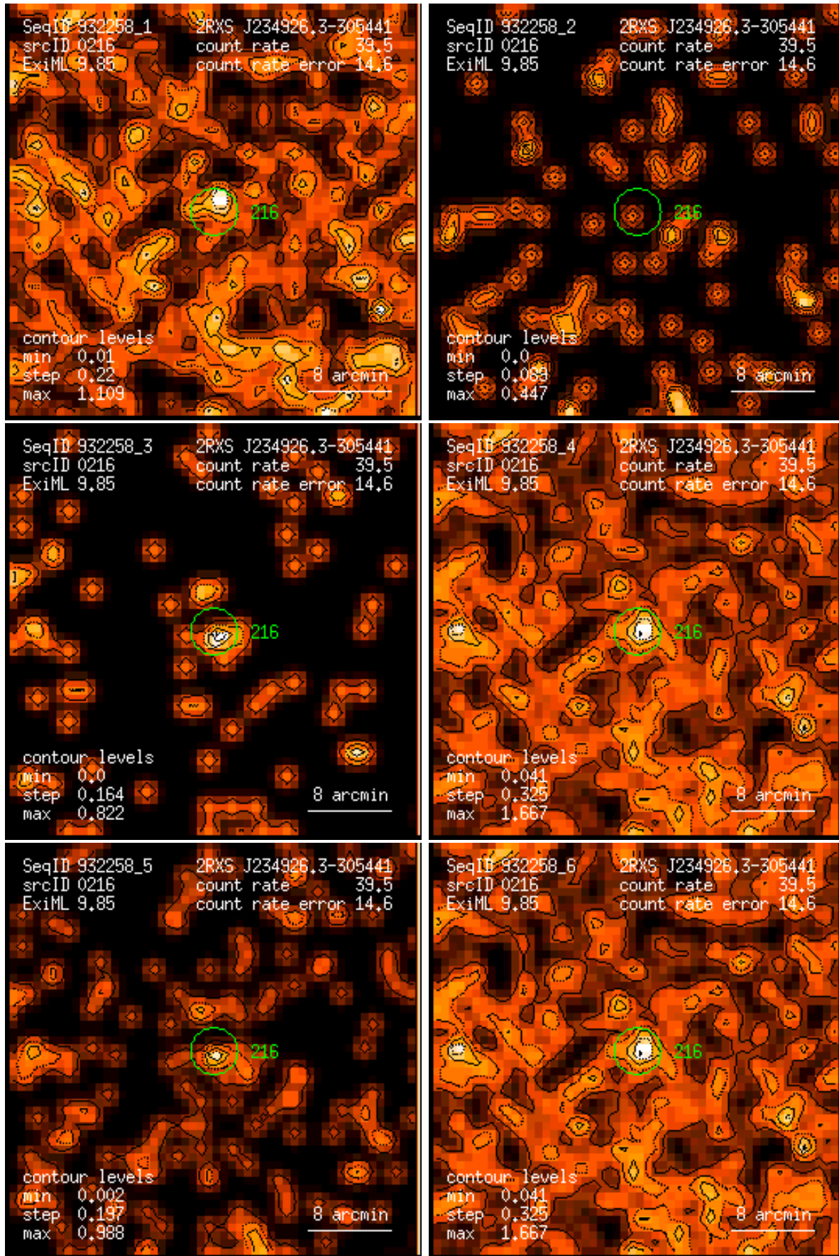
Figure 216: RASS 932258: detection 0216: band rate images, Gaussian filter: (1) PSPC channels 11 – 41, (2) 52 – 90, (3) 91 – 201, (4) 11 – 235, (5) 52 – 201, (6) 11 – 201. Broad band rates in counts/ks. Band rate contour levels in counts/ks/arcmin 2 .
