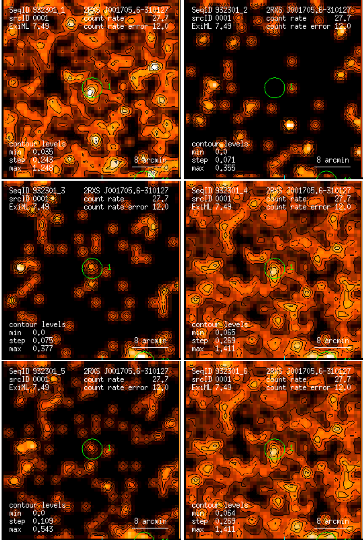
Figure 1: RASS 932301: detection 0001: band rate images, Gaussian filter: (1) PSPC channels 11 – 41, (2) 52 – 90, (3) 91 – 201, (4) 11 – 235, (5) 52 – 201, (6) 11 – 201. Broad band rates in counts/ks. Band rate contour levels in counts/ks/arcmin 2 .
