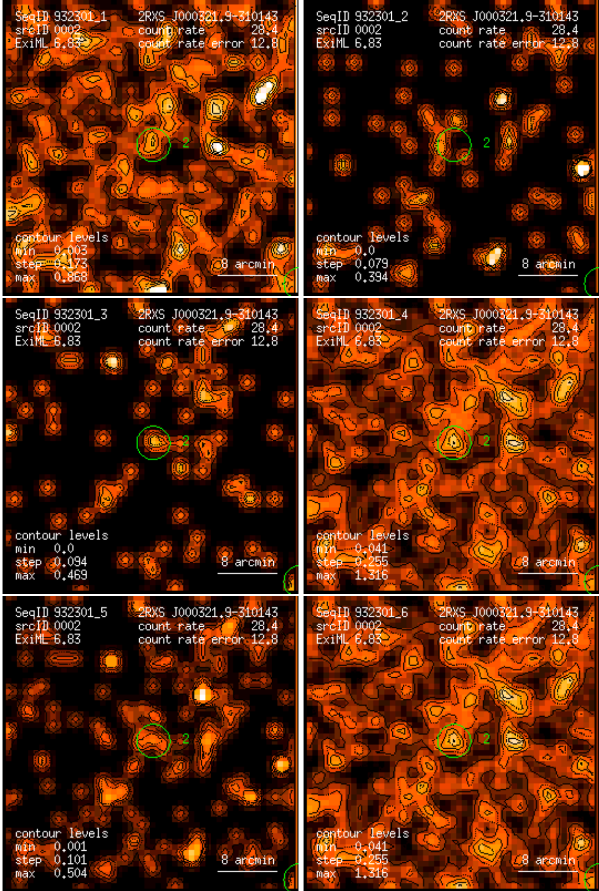
Figure 2: RASS 932301: detection 0002: band rate images, Gaussian filter: (1) PSPC channels 11 – 41, (2) 52 – 90, (3) 91 – 201, (4) 11 – 235, (5) 52 – 201, (6) 11 – 201. Broad band rates in counts/ks. Band rate contour levels in counts/ks/arcmin 2 .
