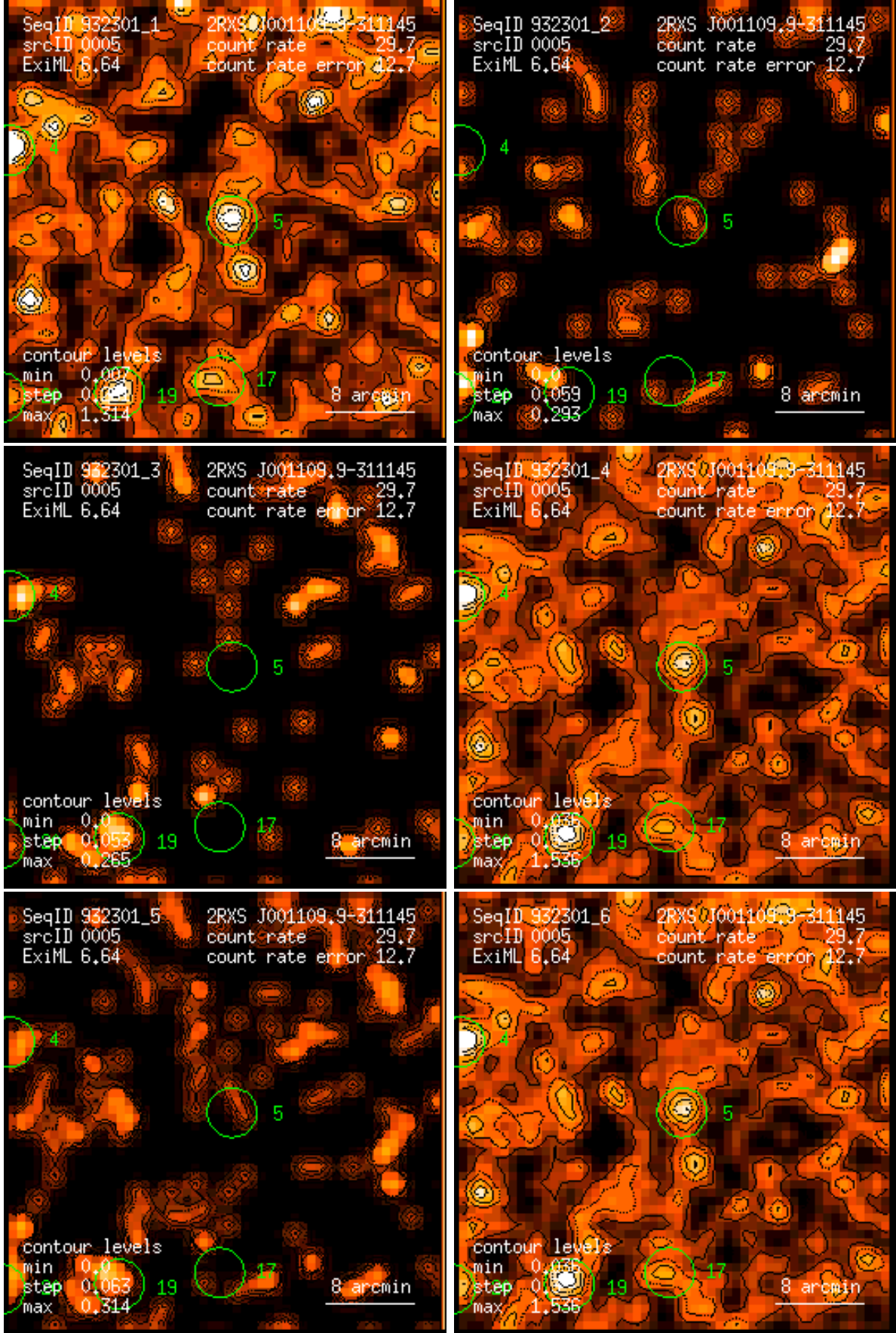
Figure 5: RASS 932301: detection 0005: band rate images, Gaussian filter: (1) PSPC channels 11 – 41, (2) 52 – 90, (3) 91 – 201, (4) 11 – 235, (5) 52 – 201, (6) 11 – 201. Broad band rates in counts/ks. Band rate contour levels in counts/ks/arcmin 2 .
