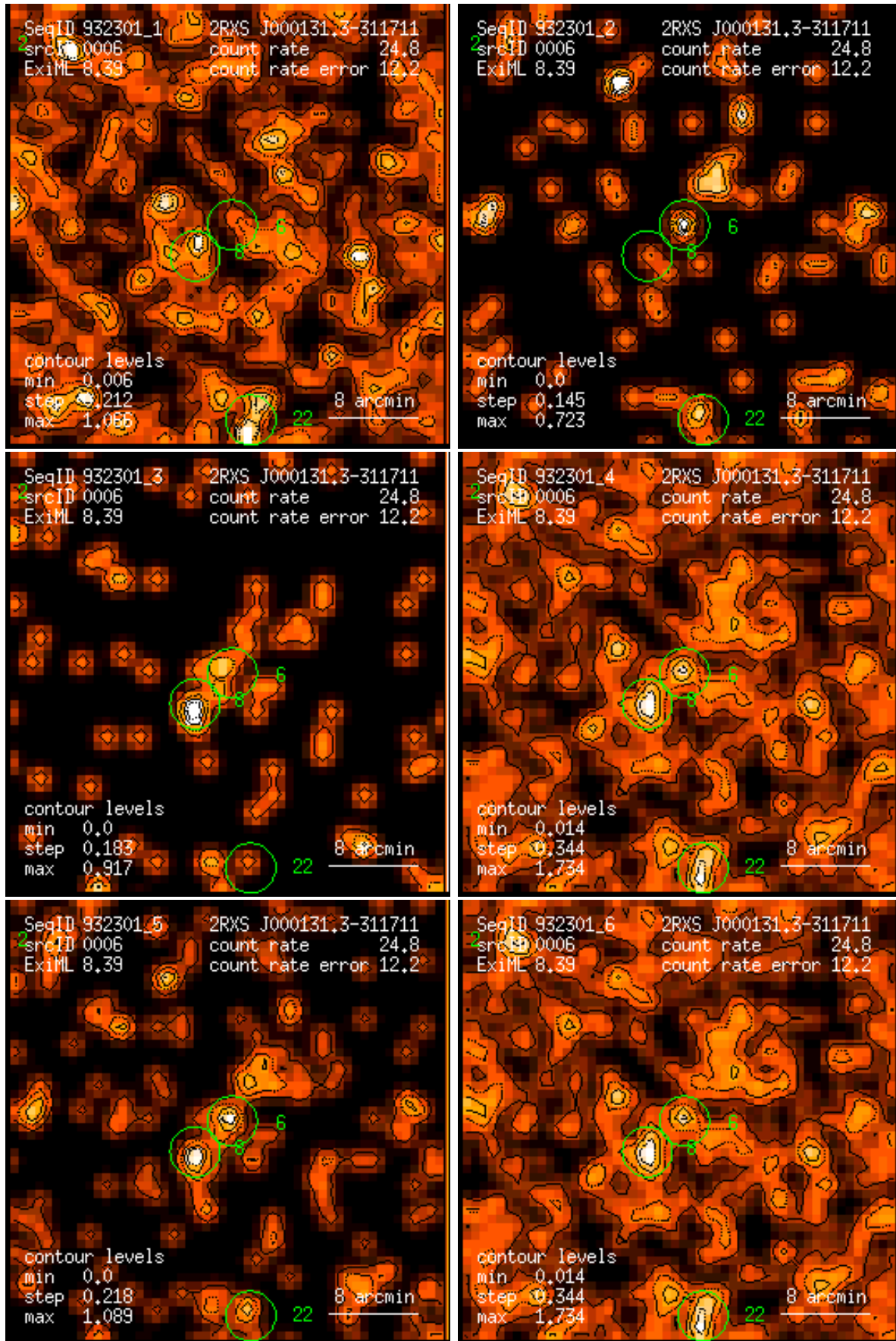
Figure 6: RASS 932301: detection 0006: band rate images, Gaussian filter: (1) PSPC channels 11 – 41, (2) 52 – 90, (3) 91 – 201, (4) 11 – 235, (5) 52 – 201, (6) 11 – 201. Broad band rates in counts/ks. Band rate contour levels in counts/ks/arcmin 2 .
