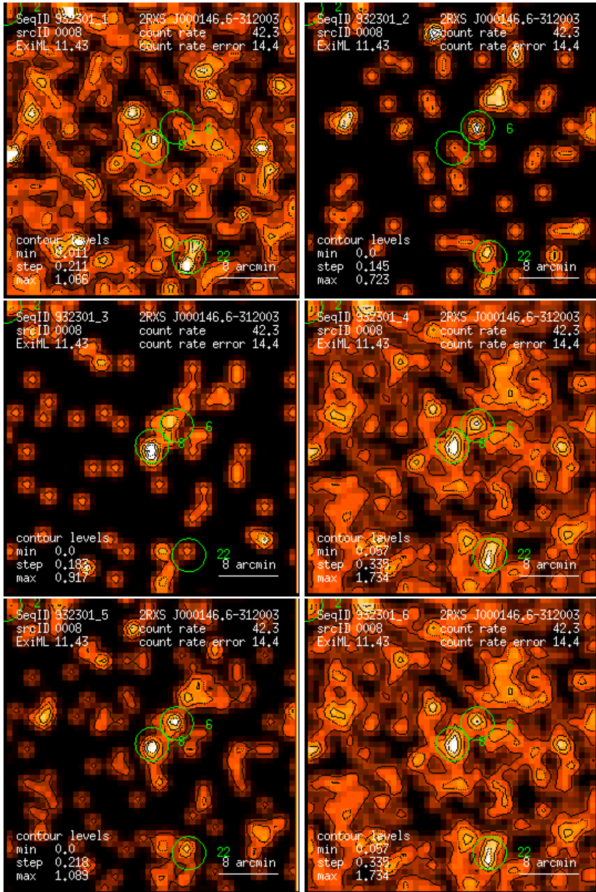
Figure 8: RASS 932301: detection 0008: band rate images, Gaussian filter: (1) PSPC channels 11 – 41, (2) 52 – 90, (3) 91 – 201, (4) 11 – 235, (5) 52 – 201, (6) 11 – 201. Broad band rates in counts/ks. Band rate contour levels in counts/ks/arcmin 2 .
