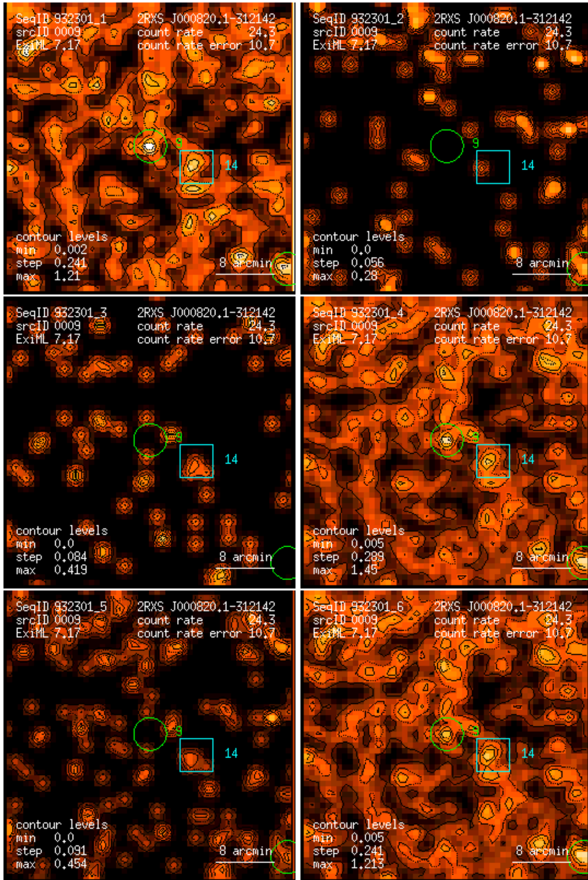
Figure 9: RASS 932301: detection 0009: band rate images, Gaussian filter: (1) PSPC channels 11 – 41, (2) 52 – 90, (3) 91 – 201, (4) 11 – 235, (5) 52 – 201, (6) 11 – 201. Broad band rates in counts/ks. Band rate contour levels in counts/ks/arcmin 2 .
