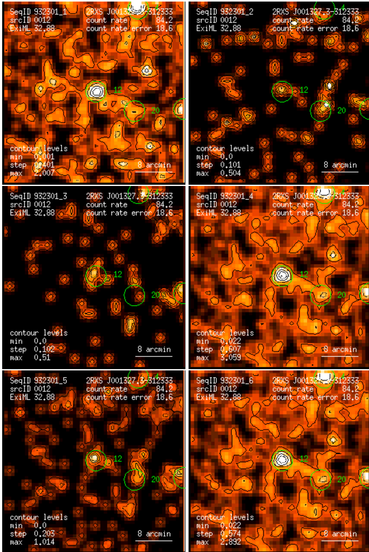
Figure 12: RASS 932301: detection 0012: band rate images, Gaussian filter: (1) PSPC channels 11 – 41, (2) 52 – 90, (3) 91 – 201, (4) 11 – 235, (5) 52 – 201, (6) 11 – 201. Broad band rates in counts/ks. Band rate contour levels in counts/ks/arcmin 2 .
