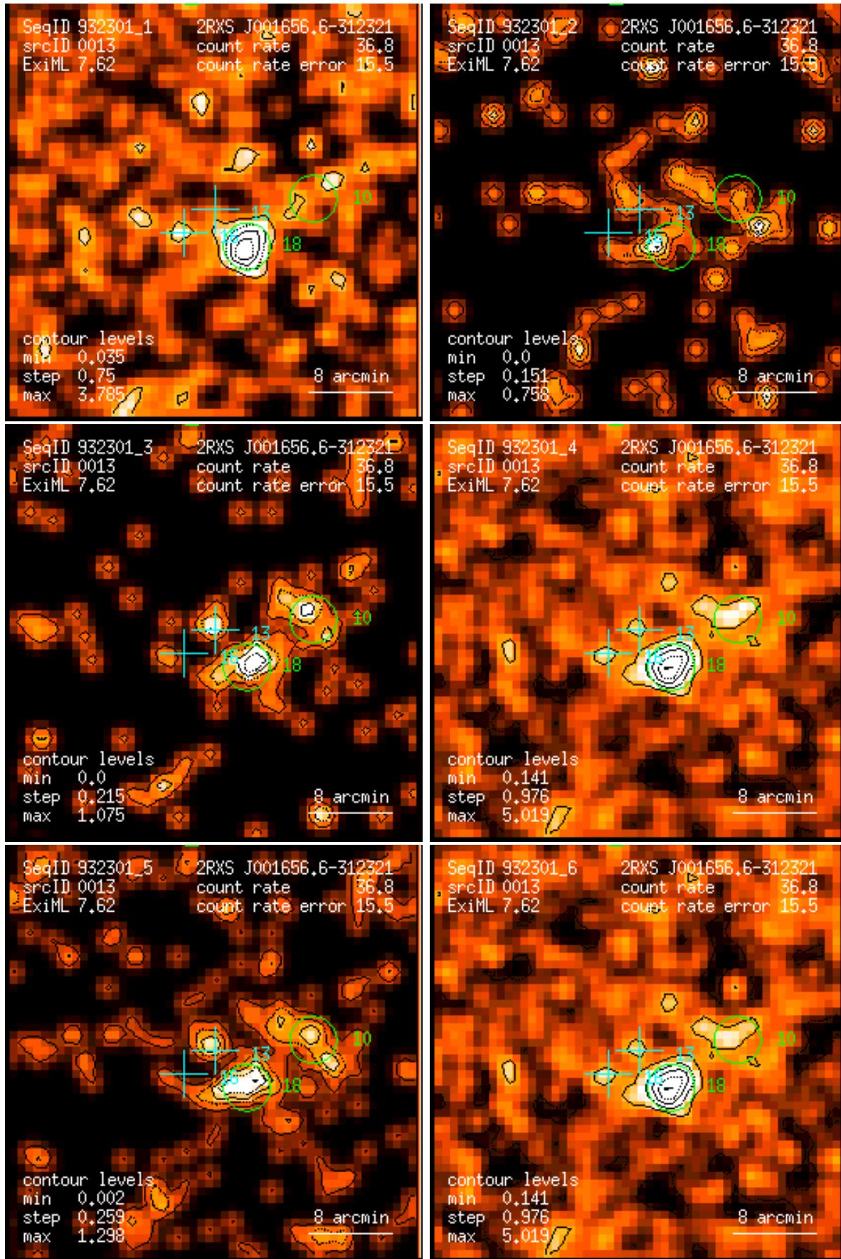
Figure 13: RASS 932301: detection 0013: band rate images, Gaussian filter: (1) PSPC channels 11 – 41, (2) 52 – 90, (3) 91 – 201, (4) 11 – 235, (5) 52 – 201, (6) 11 – 201. Broad band rates in counts/ks. Band rate contour levels in counts/ks/arcmin 2 .
