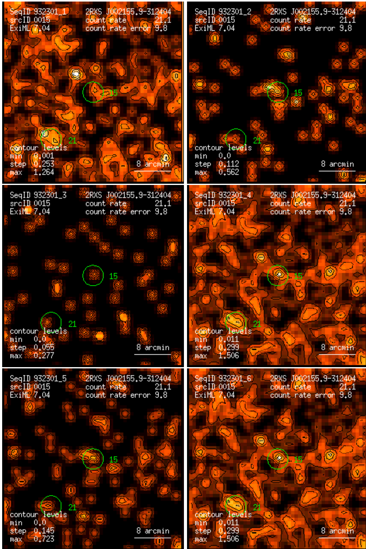
Figure 15: RASS 932301: detection 0015: band rate images, Gaussian filter: (1) PSPC channels 11 – 41, (2) 52 – 90, (3) 91 – 201, (4) 11 – 235, (5) 52 – 201, (6) 11 – 201. Broad band rates in counts/ks. Band rate contour levels in counts/ks/arcmin 2 .
