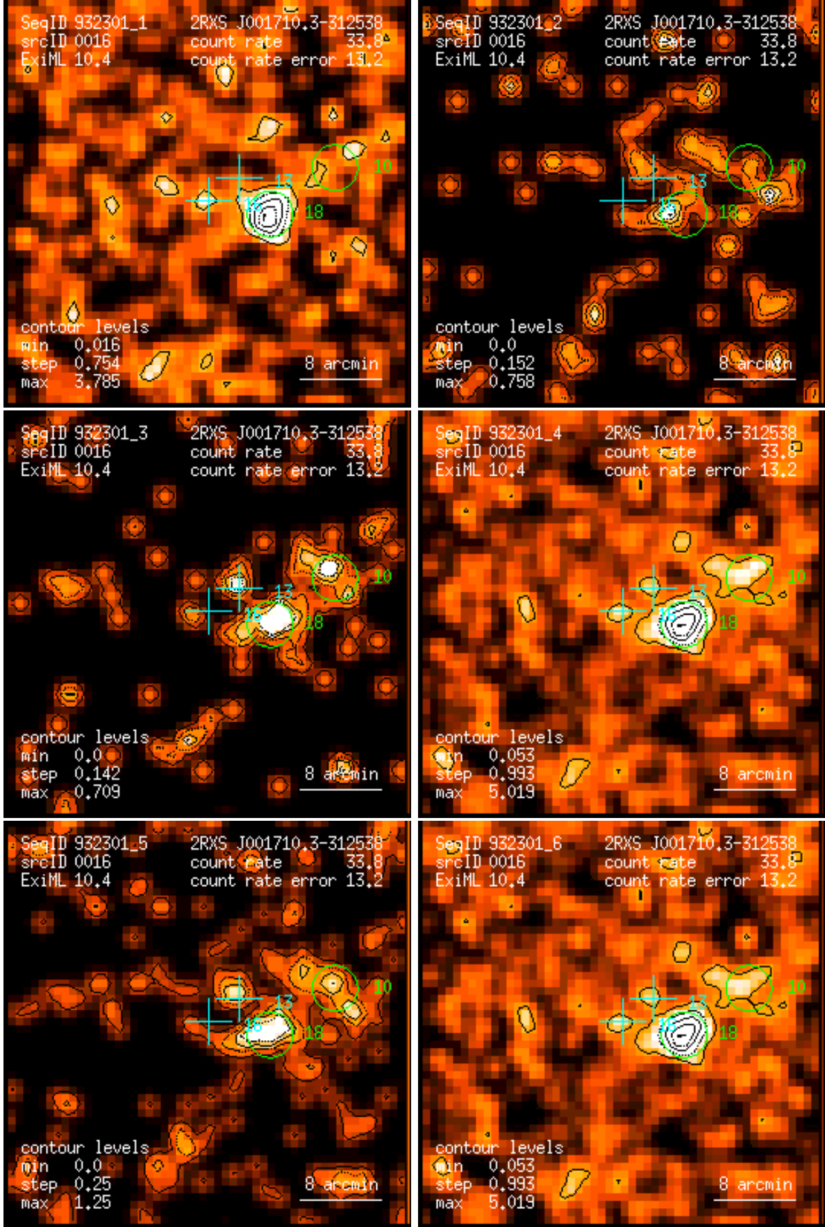
Figure 16: RASS 932301: detection 0016: band rate images, Gaussian filter: (1) PSPC channels 11 – 41, (2) 52 – 90, (3) 91 – 201, (4) 11 – 235, (5) 52 – 201, (6) 11 – 201. Broad band rates in counts/ks. Band rate contour levels in counts/ks/arcmin 2 .
