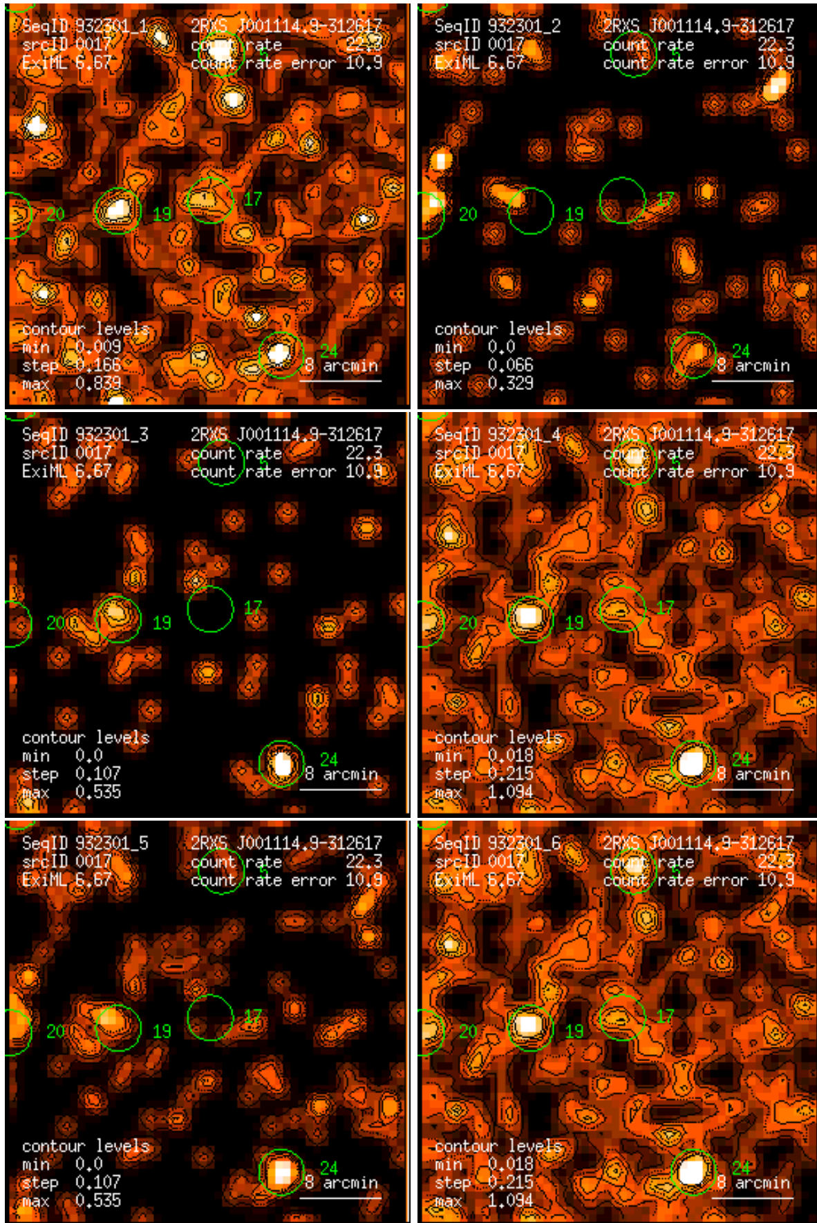
Figure 17: RASS 932301: detection 0017: band rate images, Gaussian filter: (1) PSPC channels 11 – 41, (2) 52 – 90, (3) 91 – 201, (4) 11 – 235, (5) 52 – 201, (6) 11 – 201. Broad band rates in counts/ks. Band rate contour levels in counts/ks/arcmin 2 .
