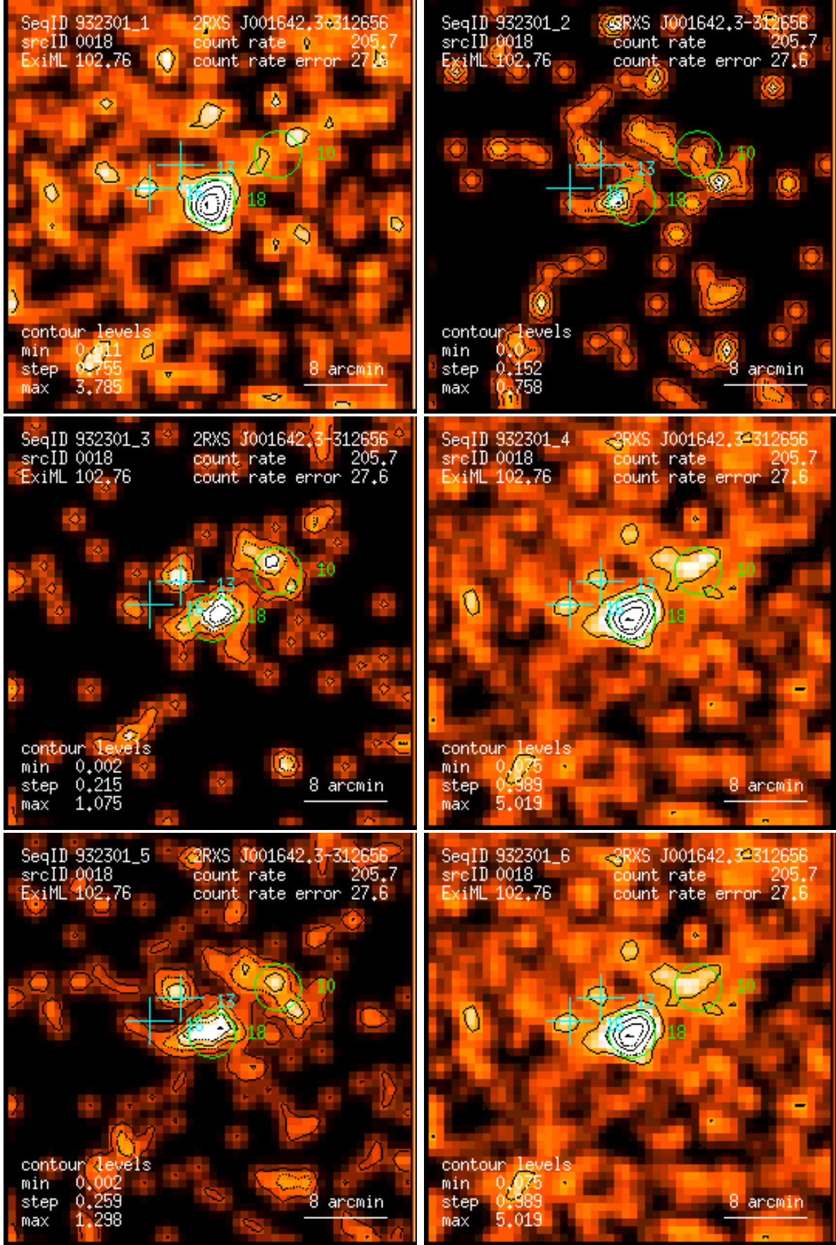
Figure 18: RASS 932301: detection 0018: band rate images, Gaussian filter: (1) PSPC channels 11 – 41, (2) 52 – 90, (3) 91 – 201, (4) 11 – 235, (5) 52 – 201, (6) 11 – 201. Broad band rates in counts/ks. Band rate contour levels in counts/ks/arcmin 2 .
