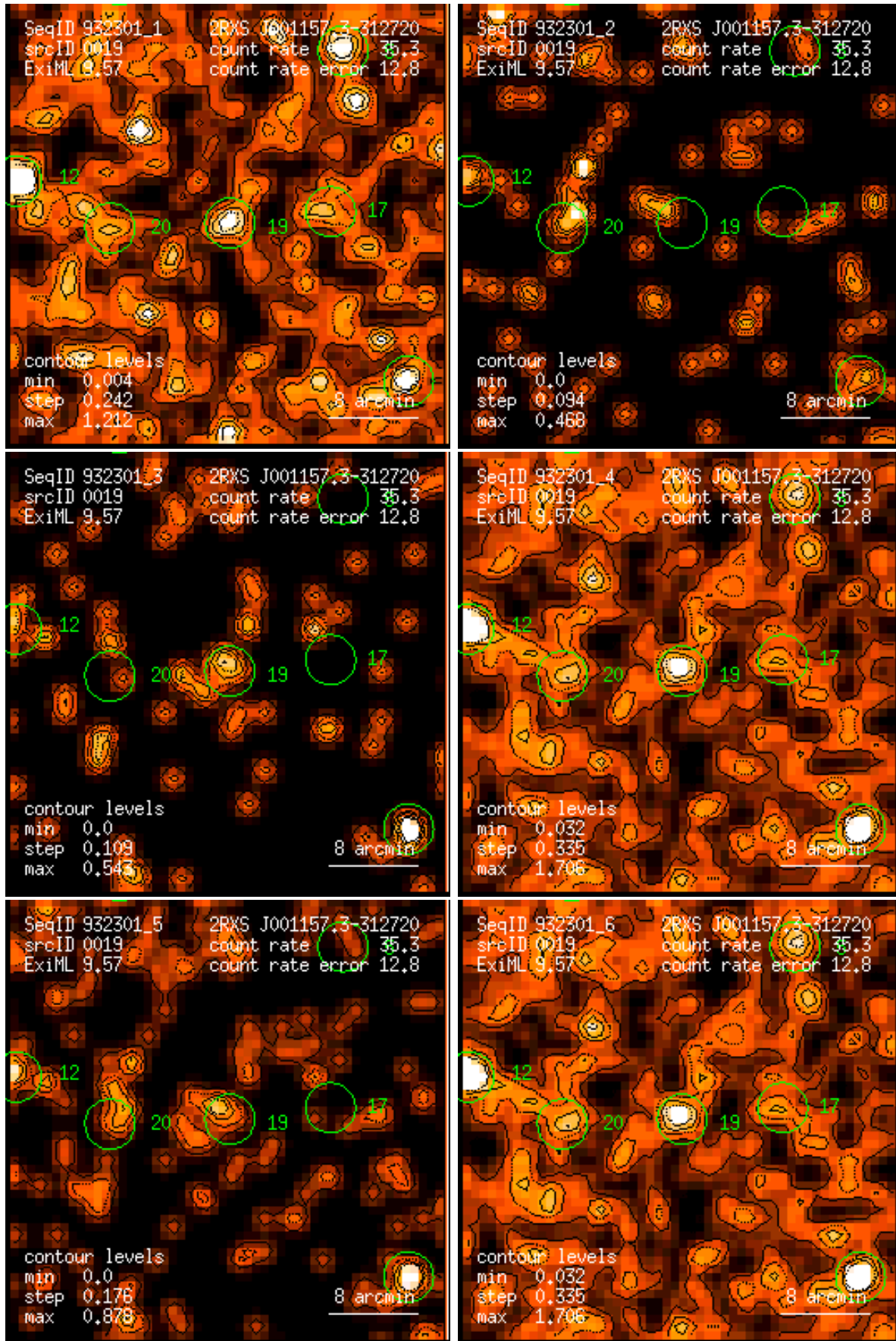
Figure 19: RASS 932301: detection 0019: band rate images, Gaussian filter: (1) PSPC channels 11 – 41, (2) 52 – 90, (3) 91 – 201, (4) 11 – 235, (5) 52 – 201, (6) 11 – 201. Broad band rates in counts/ks. Band rate contour levels in counts/ks/arcmin 2 .
