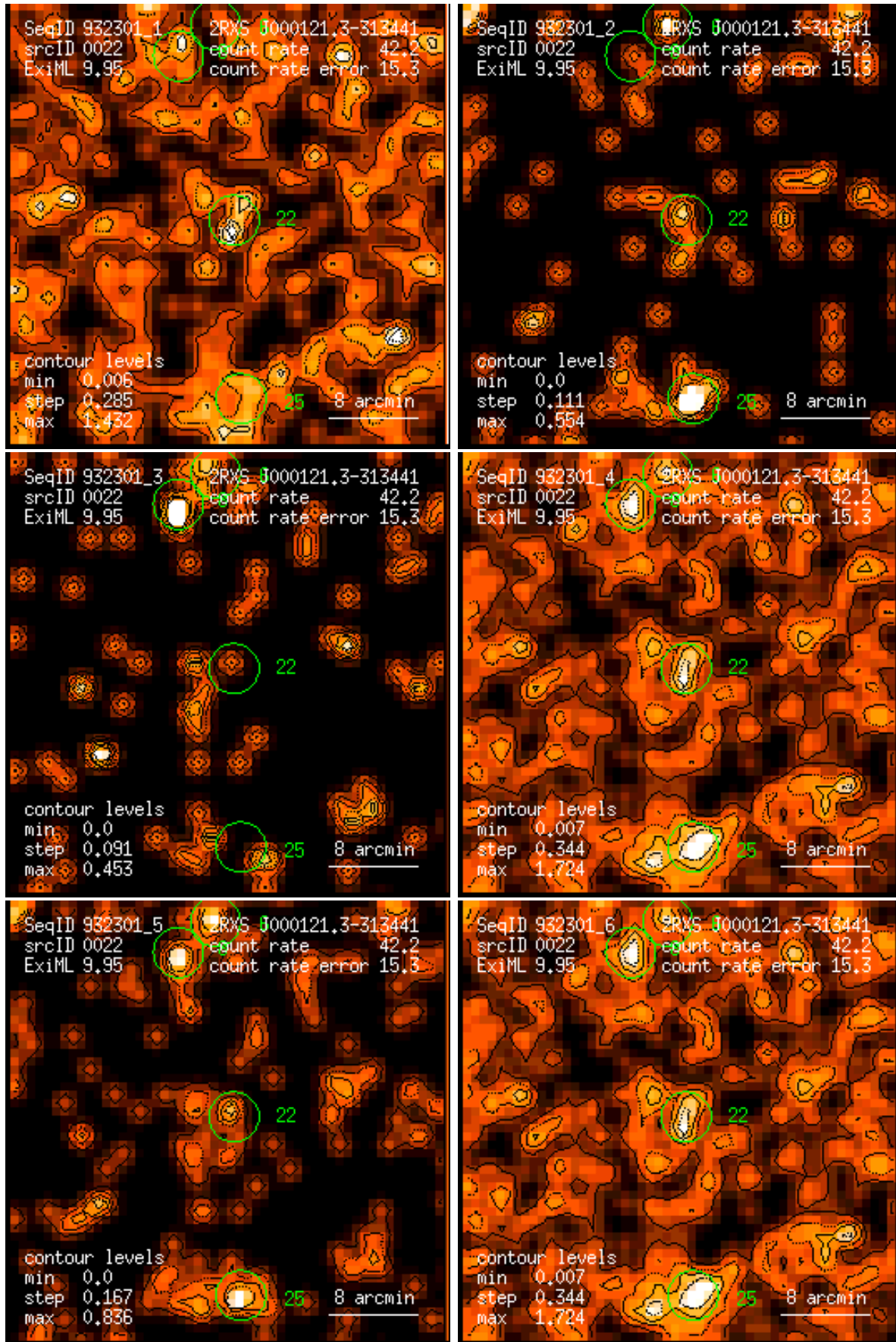
Figure 22: RASS 932301: detection 0022: band rate images, Gaussian filter: (1) PSPC channels 11 – 41, (2) 52 – 90, (3) 91 – 201, (4) 11 – 235, (5) 52 – 201, (6) 11 – 201. Broad band rates in counts/ks. Band rate contour levels in counts/ks/arcmin 2 .
