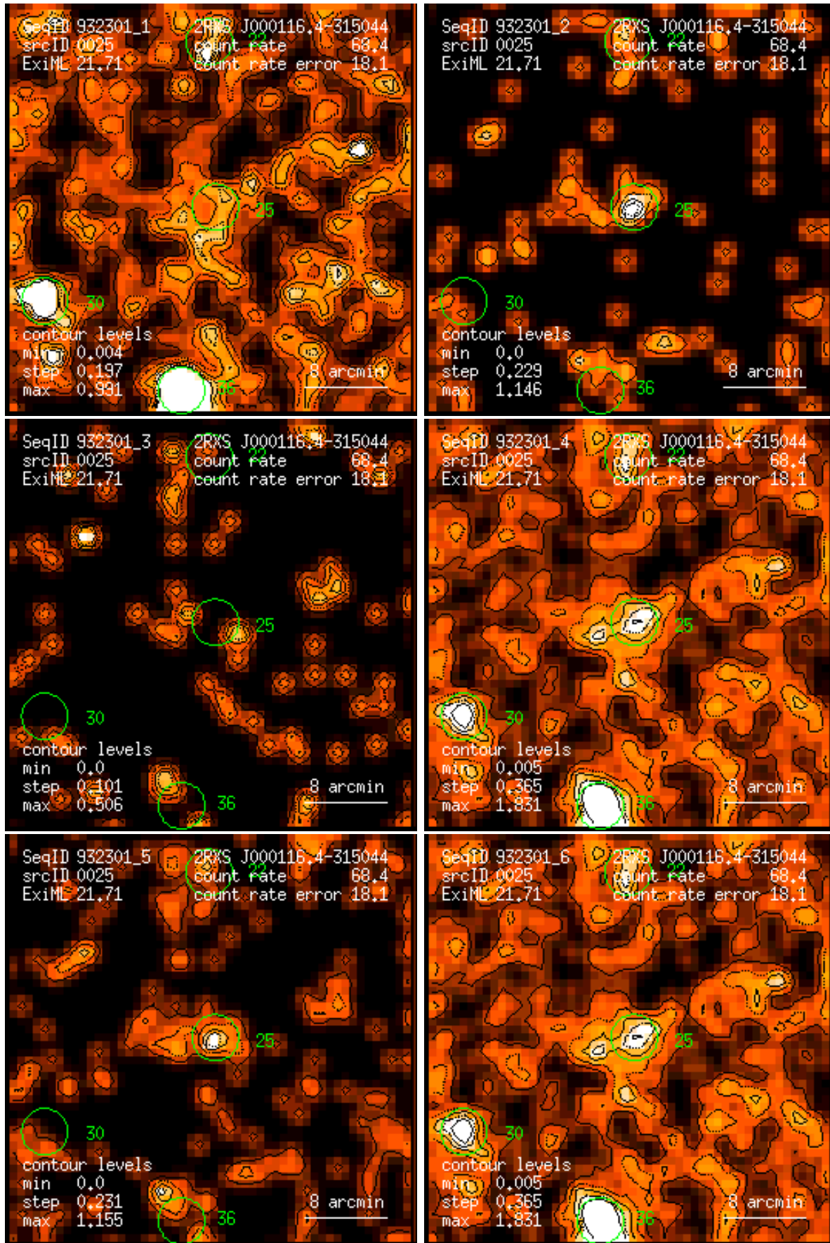
Figure 25: RASS 932301: detection 0025: band rate images, Gaussian filter: (1) PSPC channels 11 – 41, (2) 52 – 90, (3) 91 – 201, (4) 11 – 235, (5) 52 – 201, (6) 11 – 201. Broad band rates in counts/ks. Band rate contour levels in counts/ks/arcmin 2 .
