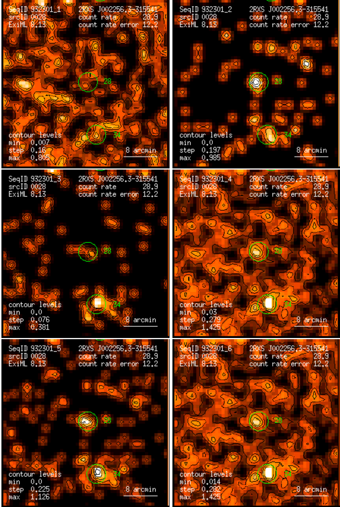
Figure 28: RASS 932301: detection 0028: band rate images, Gaussian filter: (1) PSPC channels 11 – 41, (2) 52 – 90, (3) 91 – 201, (4) 11 – 235, (5) 52 – 201, (6) 11 – 201. Broad band rates in counts/ks. Band rate contour levels in counts/ks/arcmin 2 .
