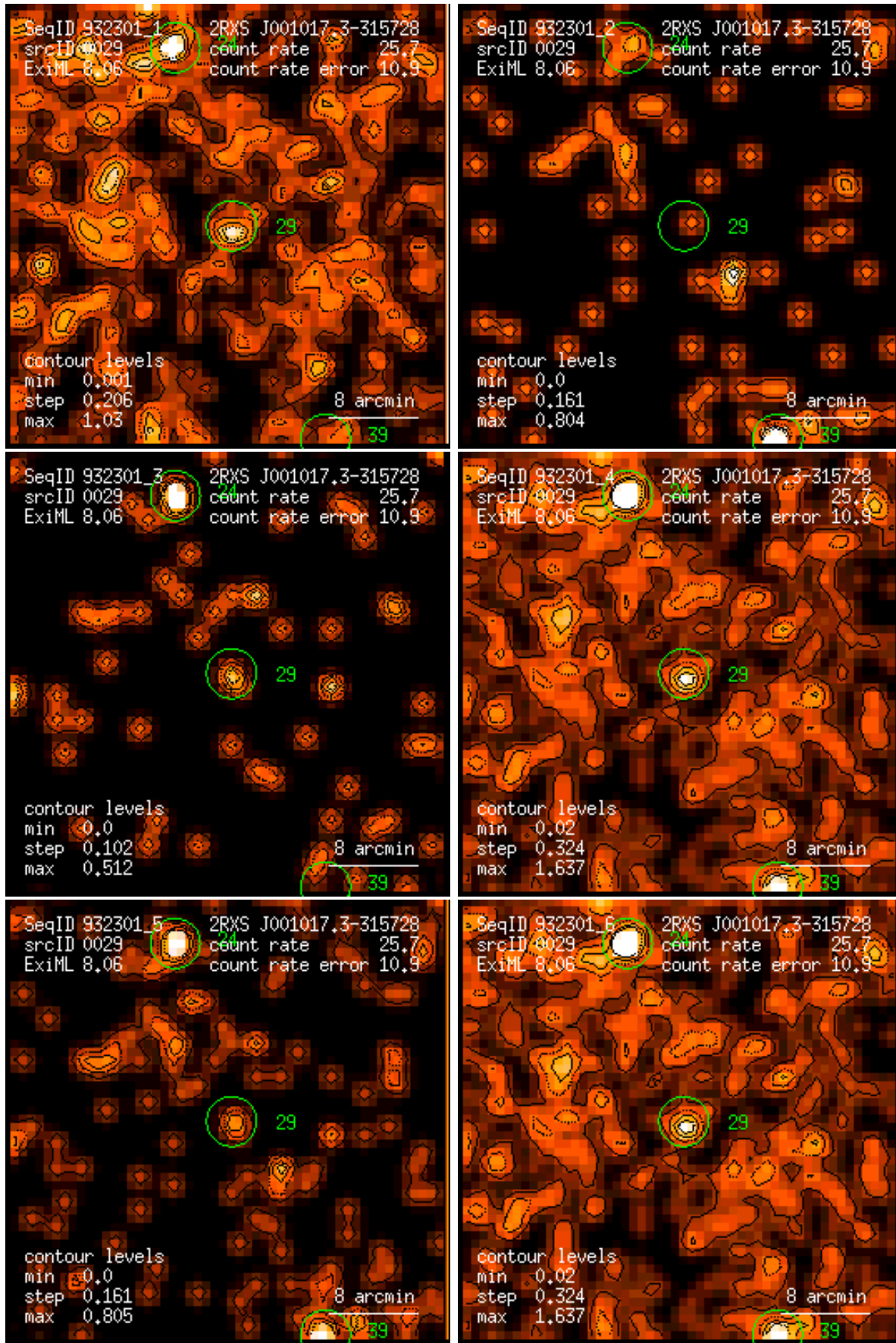
Figure 29: RASS 932301: detection 0029: band rate images, Gaussian filter: (1) PSPC channels 11 – 41, (2) 52 – 90, (3) 91 – 201, (4) 11 – 235, (5) 52 – 201, (6) 11 – 201. Broad band rates in counts/ks. Band rate contour levels in counts/ks/arcmin 2 .
