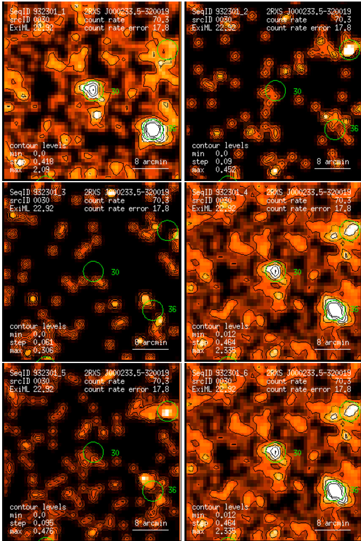
Figure 30: RASS 932301: detection 0030: band rate images, Gaussian filter: (1) PSPC channels 11 – 41, (2) 52 – 90, (3) 91 – 201, (4) 11 – 235, (5) 52 – 201, (6) 11 – 201. Broad band rates in counts/ks. Band rate contour levels in counts/ks/arcmin 2 .
