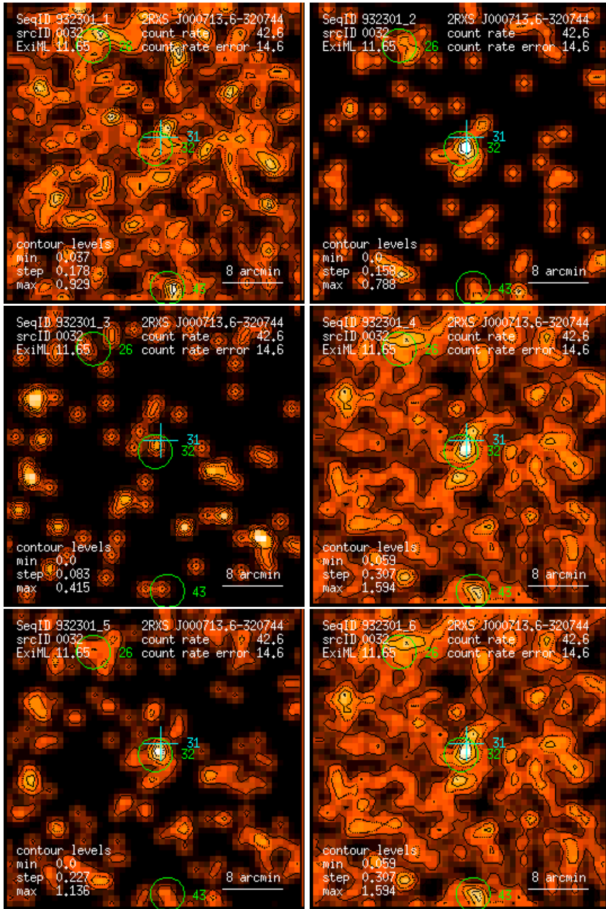
Figure 32: RASS 932301: detection 0032: band rate images, Gaussian filter: (1) PSPC channels 11 – 41, (2) 52 – 90, (3) 91 – 201, (4) 11 – 235, (5) 52 – 201, (6) 11 – 201. Broad band rates in counts/ks. Band rate contour levels in counts/ks/arcmin 2 .
