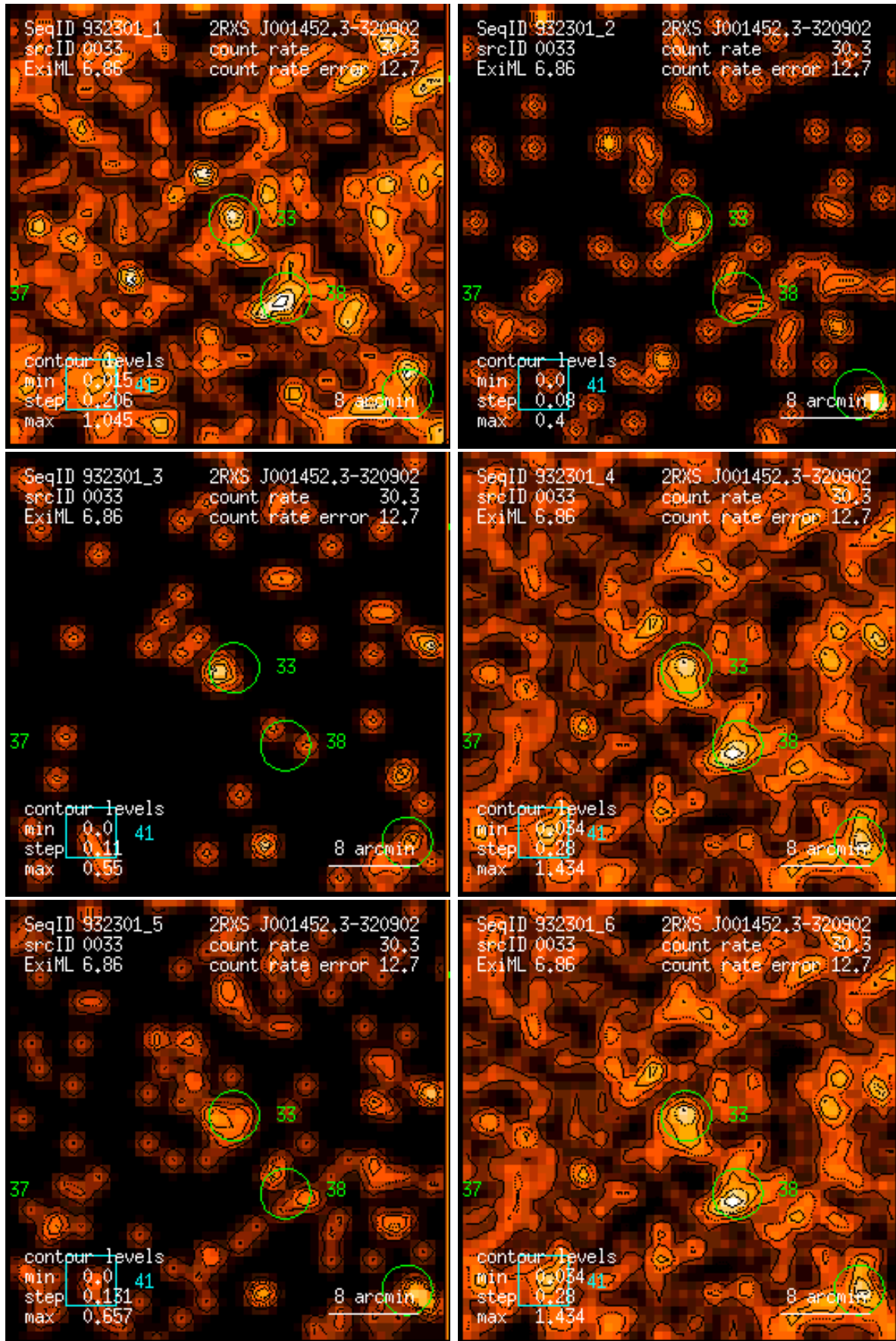
Figure 33: RASS 932301: detection 0033: band rate images, Gaussian filter: (1) PSPC channels 11 – 41, (2) 52 – 90, (3) 91 – 201, (4) 11 – 235, (5) 52 – 201, (6) 11 – 201. Broad band rates in counts/ks. Band rate contour levels in counts/ks/arcmin 2 .
