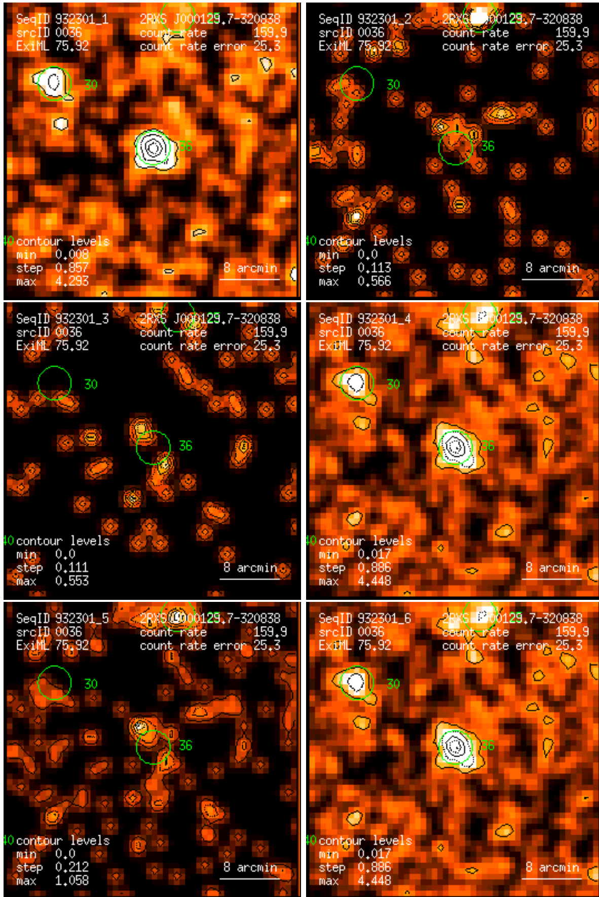
Figure 36: RASS 932301: detection 0036: band rate images, Gaussian filter: (1) PSPC channels 11 – 41, (2) 52 – 90, (3) 91 – 201, (4) 11 – 235, (5) 52 – 201, (6) 11 – 201. Broad band rates in counts/ks. Band rate contour levels in counts/ks/arcmin 2 .
