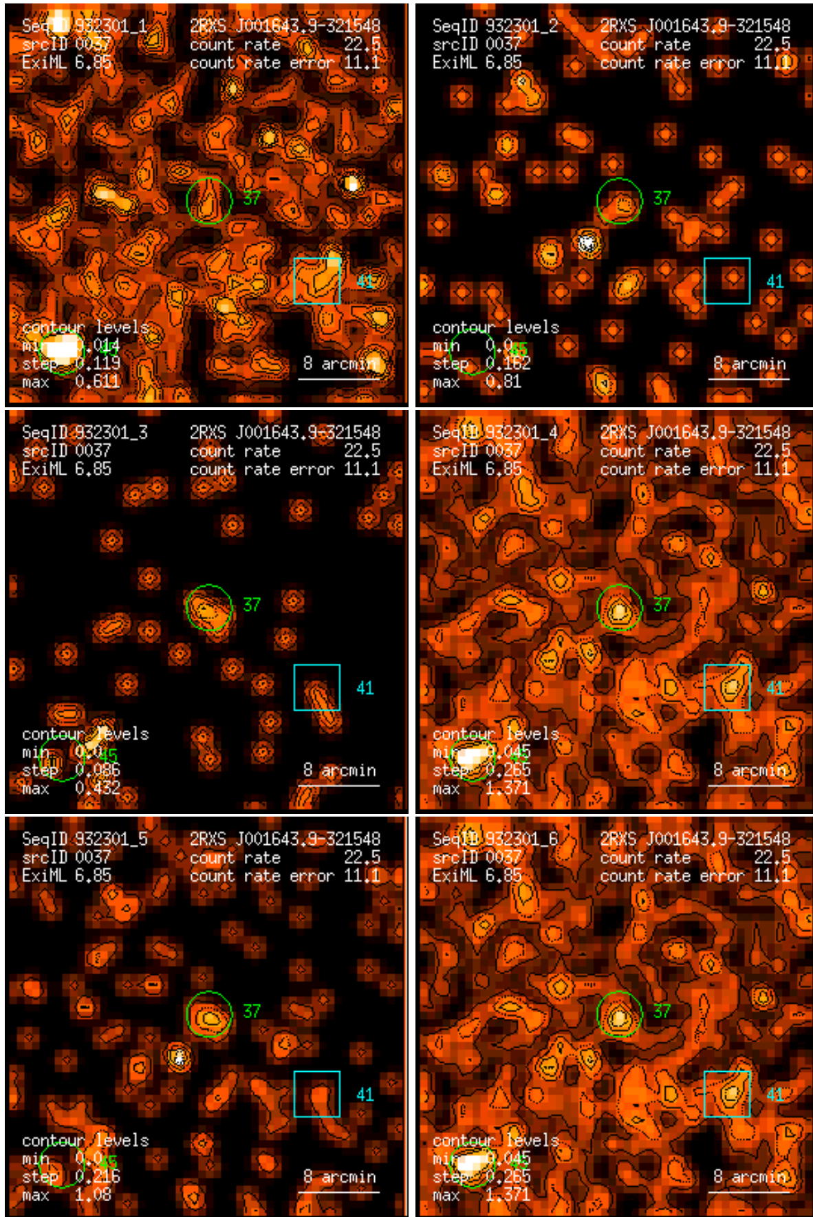
Figure 37: RASS 932301: detection 0037: band rate images, Gaussian filter: (1) PSPC channels 11 – 41, (2) 52 – 90, (3) 91 – 201, (4) 11 – 235, (5) 52 – 201, (6) 11 – 201. Broad band rates in counts/ks. Band rate contour levels in counts/ks/arcmin 2 .
