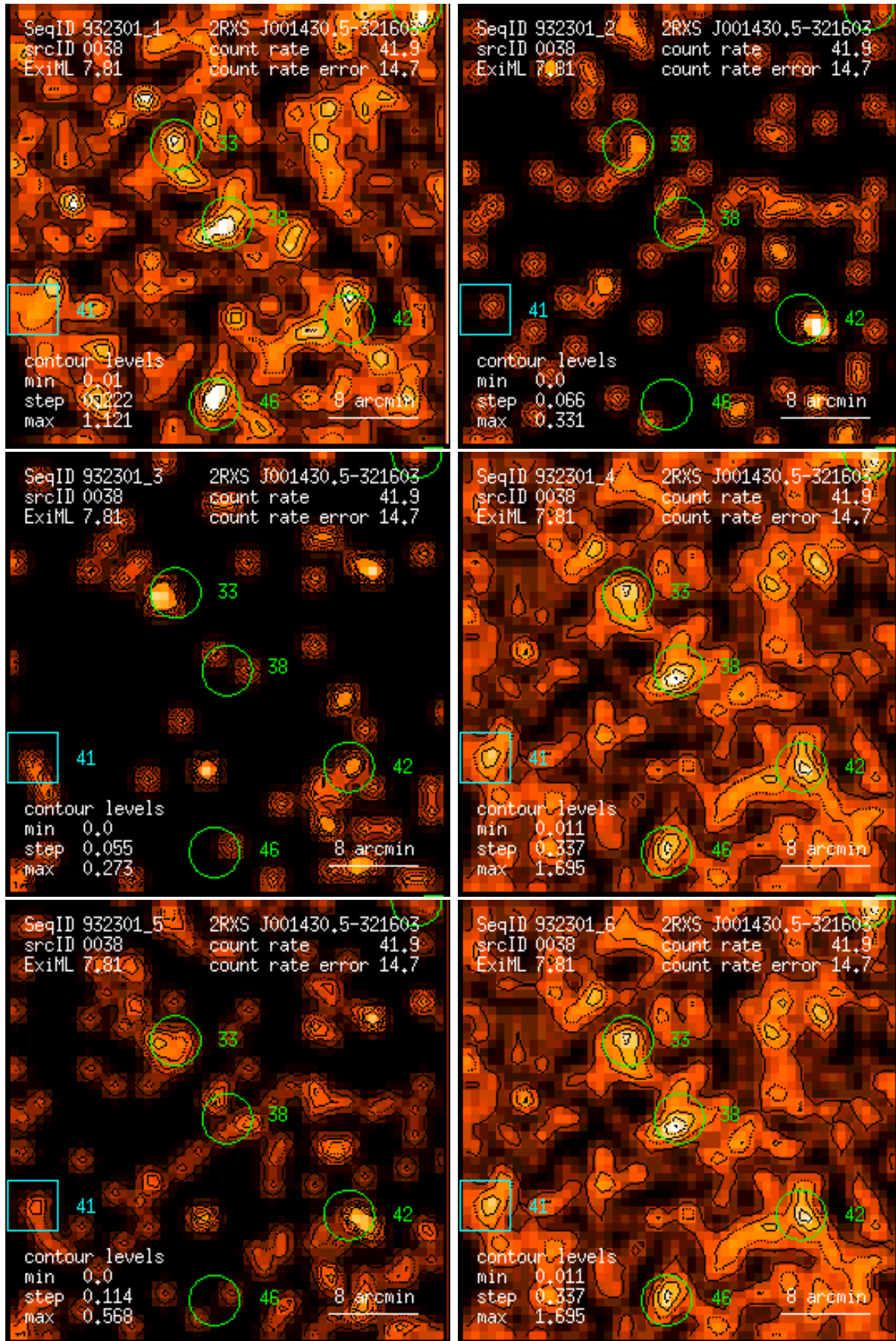
Figure 38: RASS 932301: detection 0038: band rate images, Gaussian filter: (1) PSPC channels 11 – 41, (2) 52 – 90, (3) 91 – 201, (4) 11 – 235, (5) 52 – 201, (6) 11 – 201. Broad band rates in counts/ks. Band rate contour levels in counts/ks/arcmin 2 .
